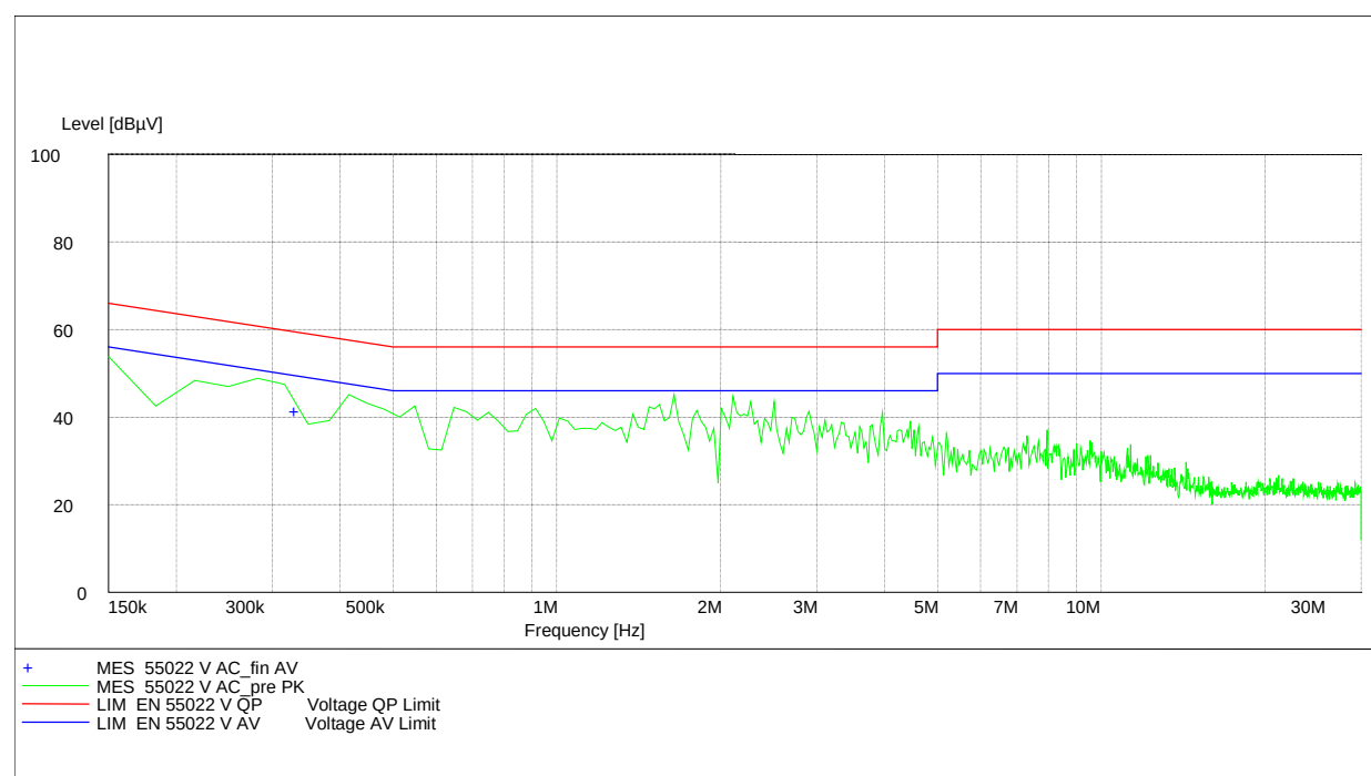
Plot 1: CISPR 22
