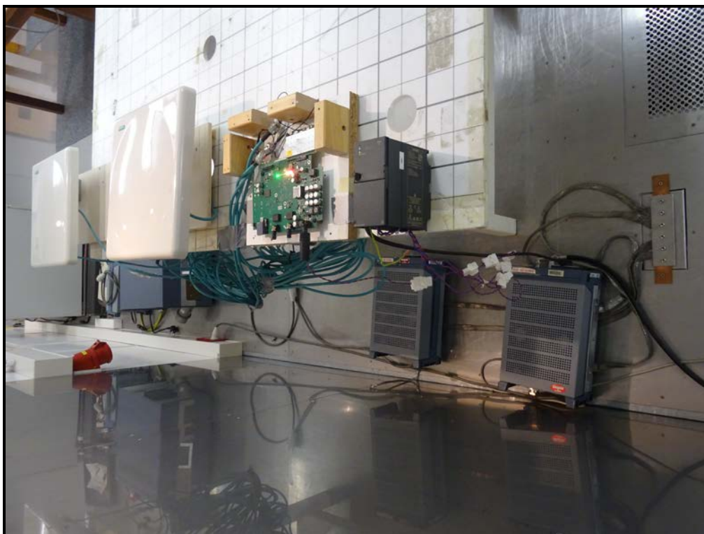
Photo 3:EUT- MIMO PORT 1+2+3+4 (No Port Terminatd with 50 \Omega )
