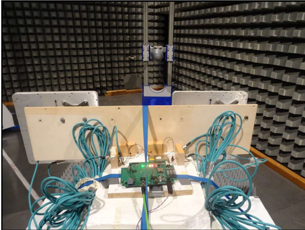
Photo 55:EUT- MIMO PORT 1+2+3+4 (No Port Terminatd with 50 \Omega )
