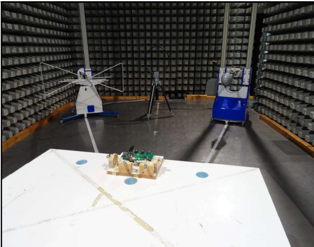
Photo 2: Terminated Ports 1+2+3+4 with 50 Ω
