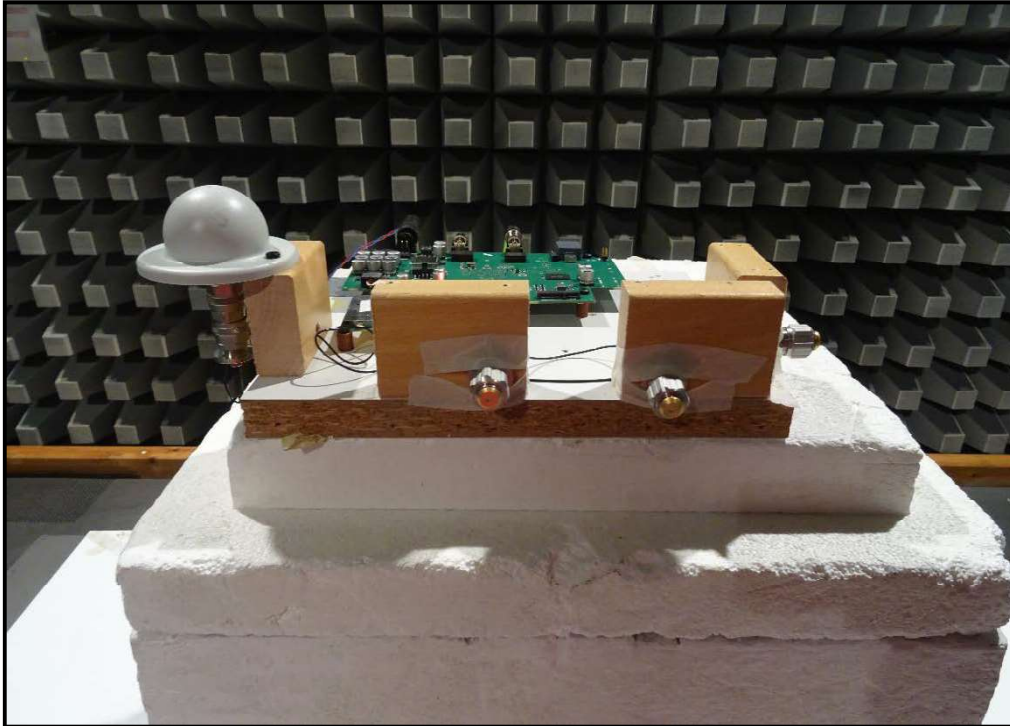
Photo 11: EUT- SISO PORT 1 (Ports 2,3 & 4 Terminated with 50 \Omega )
