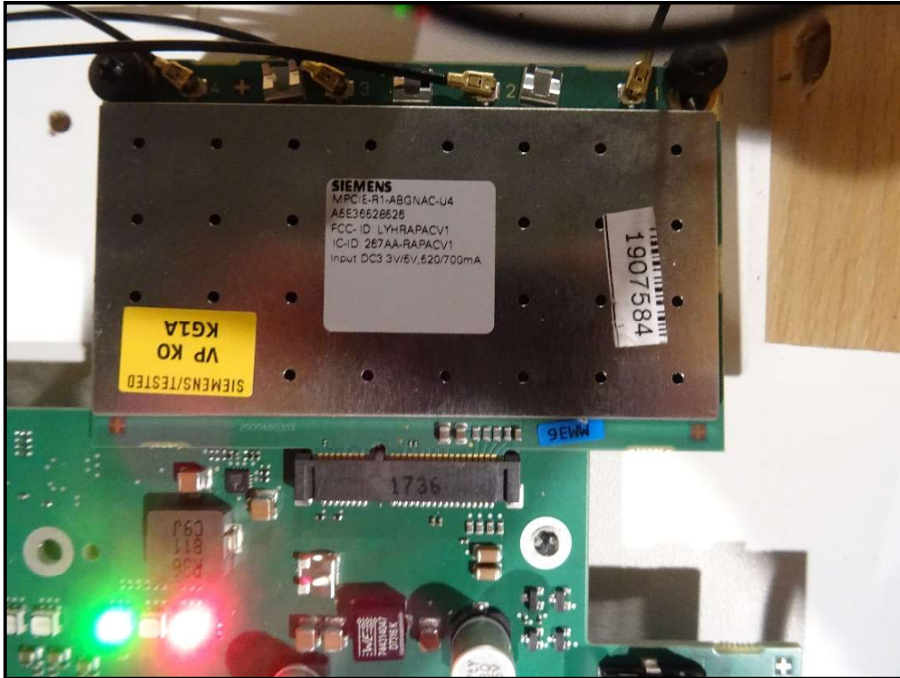
Photo 10: Terminated Ports 1+2+3+4 with 50 Ω- Radio Module Details
