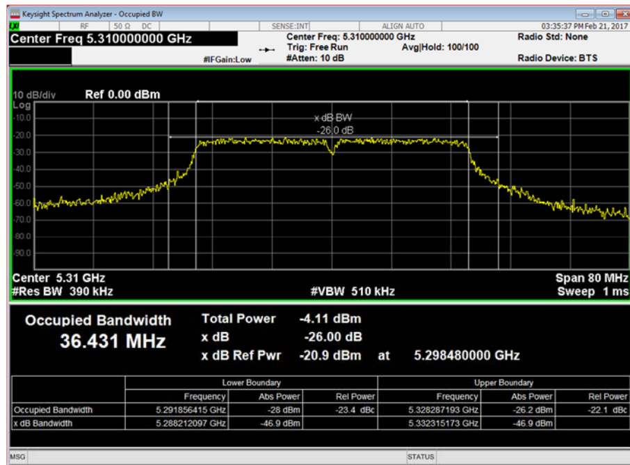
Figure 31 - Occupied Bandwidth
