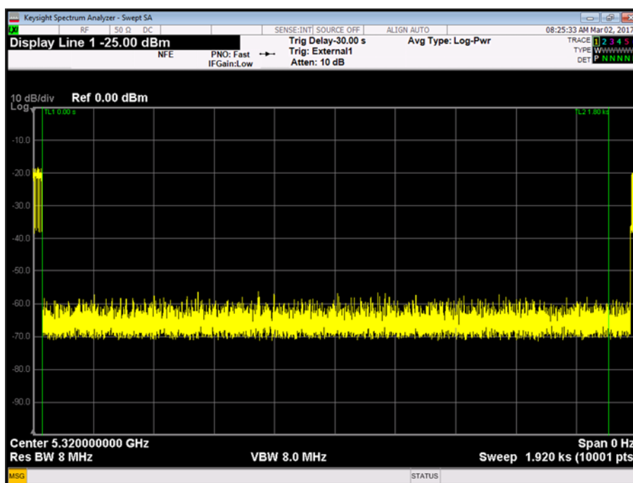
Figure 55 - Non-Occupancy Period
