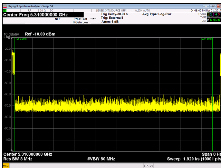
Figure 58 - Non-Occupancy Period
