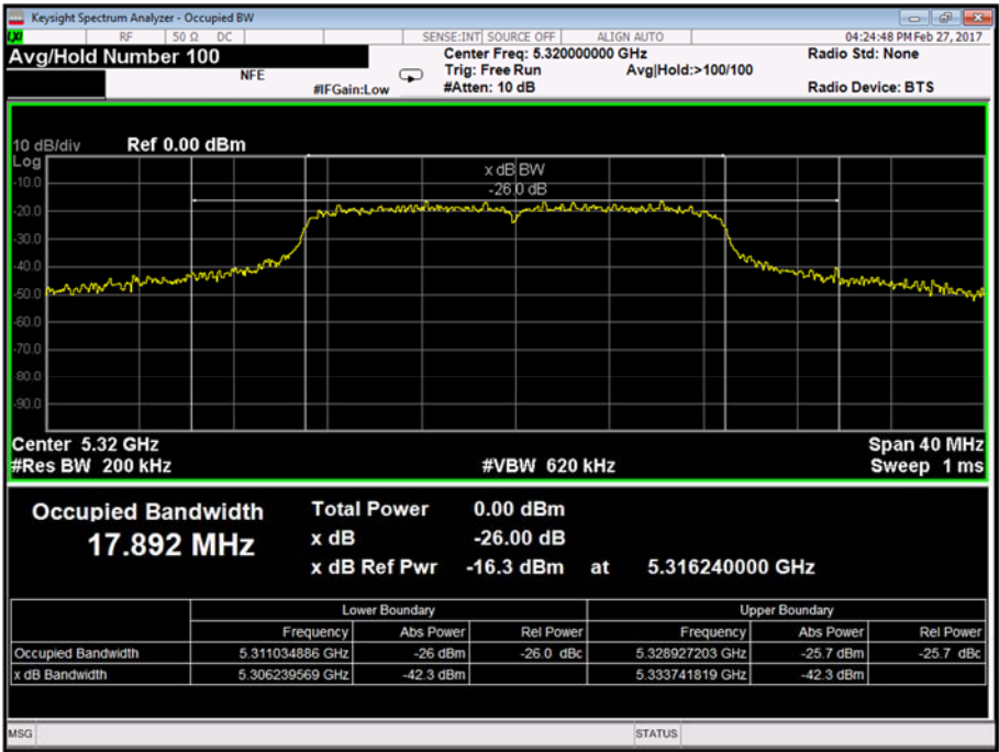
Figure 21 - Occupied Bandwidth
