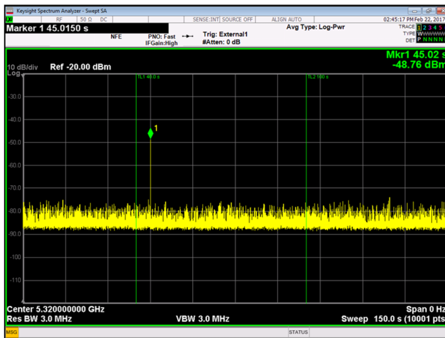
Figure 43 - Radar Injected at the Beginning of the Channel Availability Check
