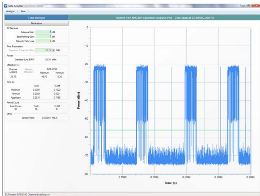
Figure 10 - Channel Loading
