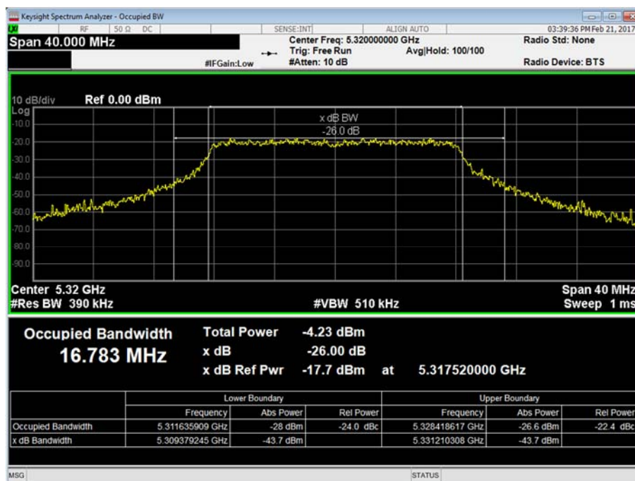
Figure 11 - Occupied Bandwidth
