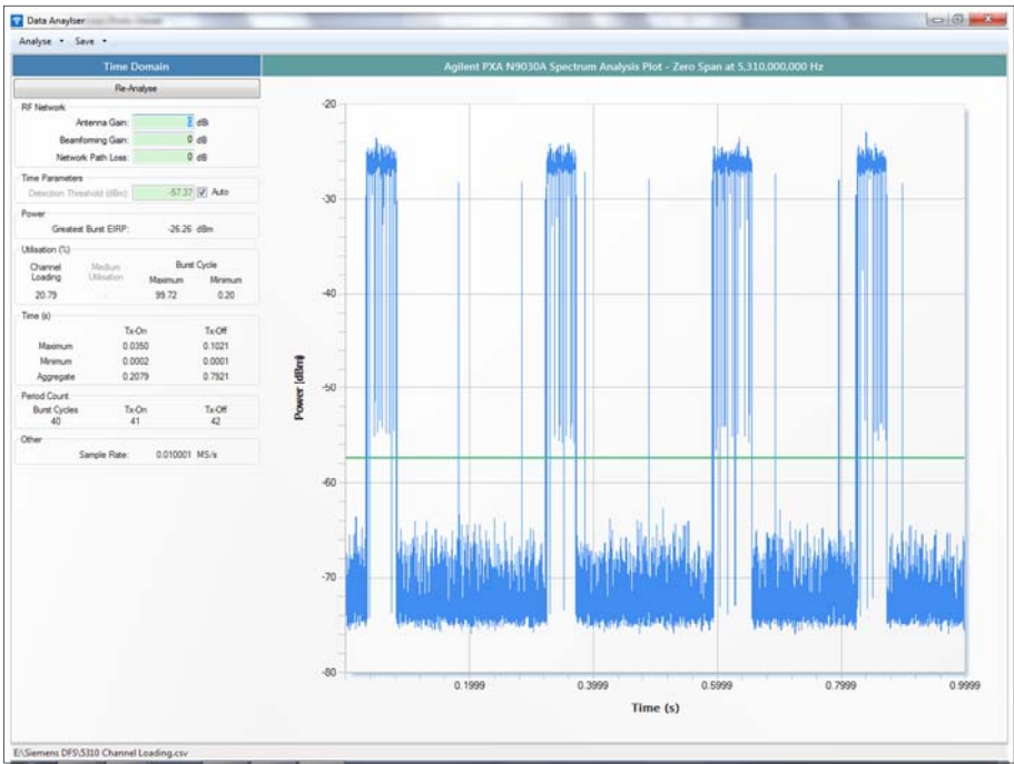
Figure 30 - Channel Loading
