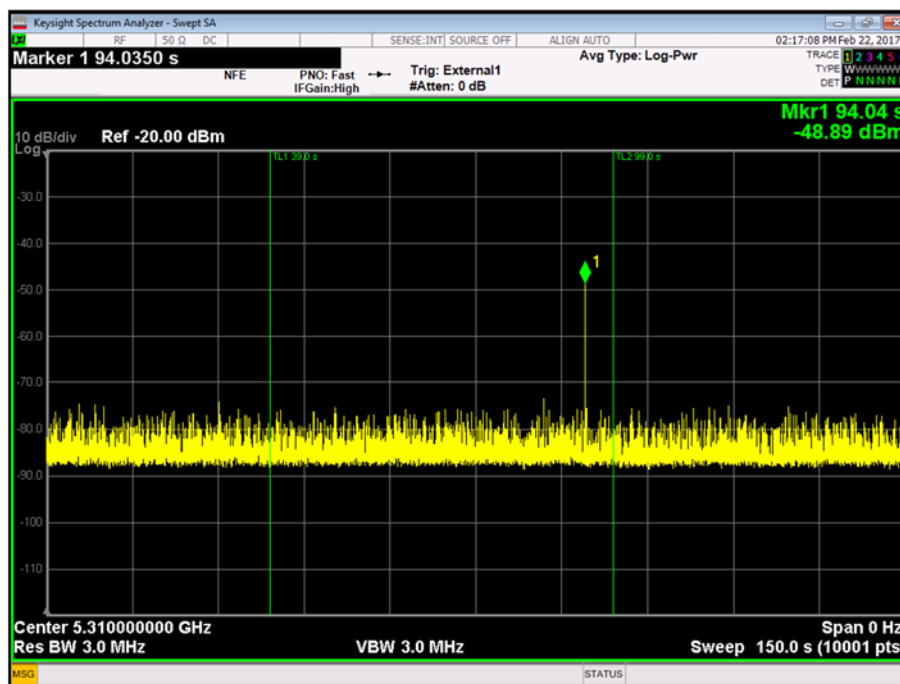
Figure 46 - Radar Injected at the end of the Channel Availability Check
