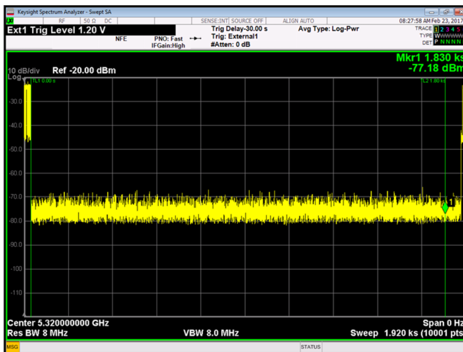
Figure 49 - Non-Occupancy Period
