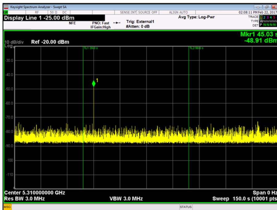
Figure 44 - Radar Injected at the Beginning of the Channel Availability Check
