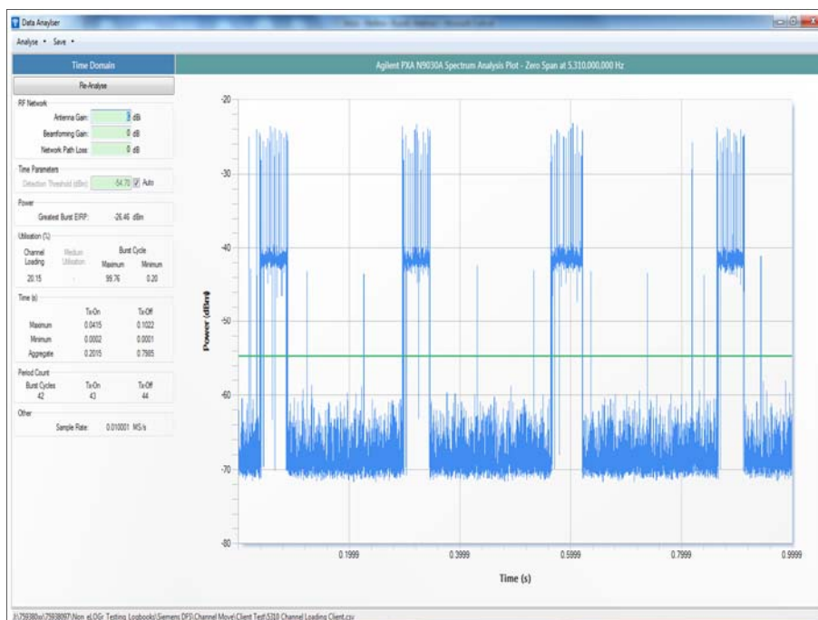
Figure 37 - Channel Loading
