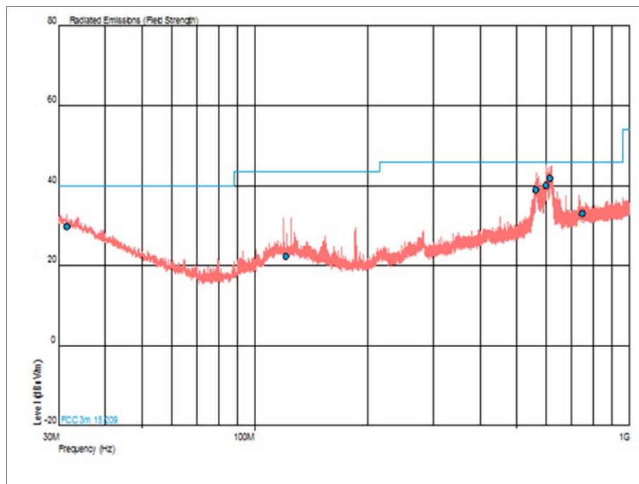
Figure 398 - U-NII 3 - 5785 MHz - 30 MHz to 1 GHz - Horizontal and Vertical
