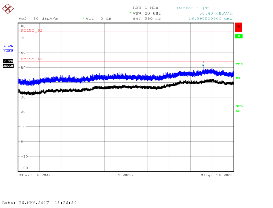
Figure 376 - U-NII 2a - 5300 MHz - 8 GHz to 18 GHz - Horizontal and Vertical
