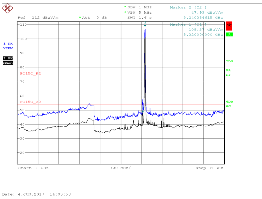
Figure 427 - U-NII 2a - 5320 MHz - 1 GHz to 8 GHz - Horizontal and Vertical
