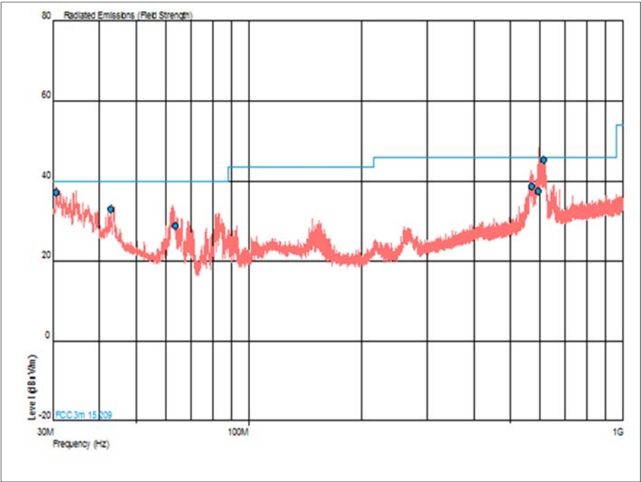
Figure 426 - U-NII 2a - 5320 MHz - 30 MHz to 1 GHz - Horizontal and Vertical
