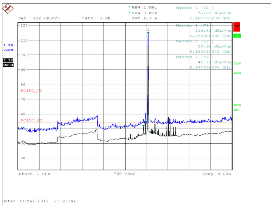
Figure 371 - U-NII 2a - 5260 MHz - 1 GHz to 8 GHz - Horizontal and Vertical
