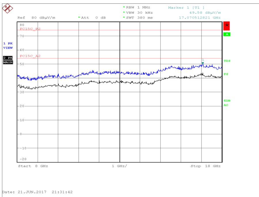
Figure 440 - U-NII 2c - 5700 MHz - 8 GHz to 18 GHz - Horizontal and Vertical
