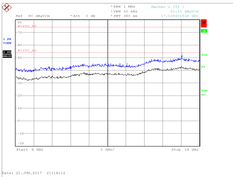
Figure 428 - U-NII 2a - 5320 MHz - 8 GHz to 18 GHz - Horizontal and Vertical
