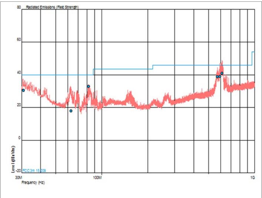
Figure 422 - U-NII 2a - 5300 MHz - 30 MHz to 1 GHz - Horizontal and Vertical
