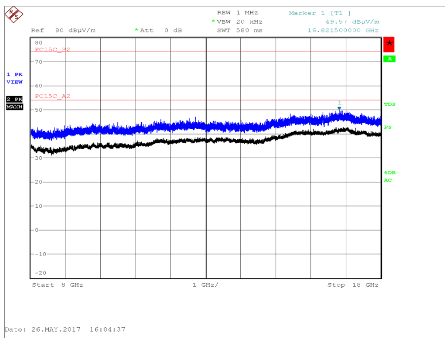
Figure 404 - U-NII 3 - 5825 MHz - 8 GHz to 18 GHz - Horizontal and Vertical
