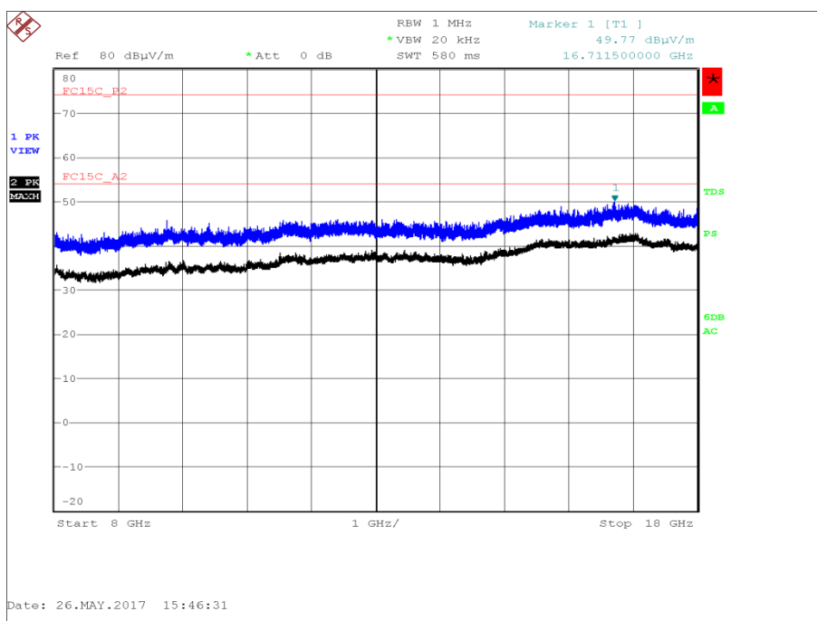
Figure 392 - U-NII 2c - 5700 MHz - 8 GHz to 18 GHz - Horizontal and Vertical
