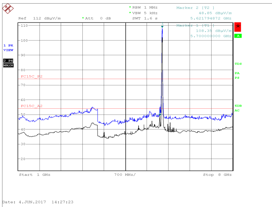
Figure 439 - U-NII 2c - 5700 MHz - 1 GHz to 8 GHz - Horizontal and Vertical
