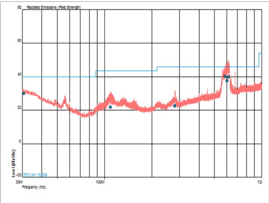
Figure 434 - U-NII 2c - 5580 MHz - 30 MHz to 1 GHz - Horizontal and Vertical
