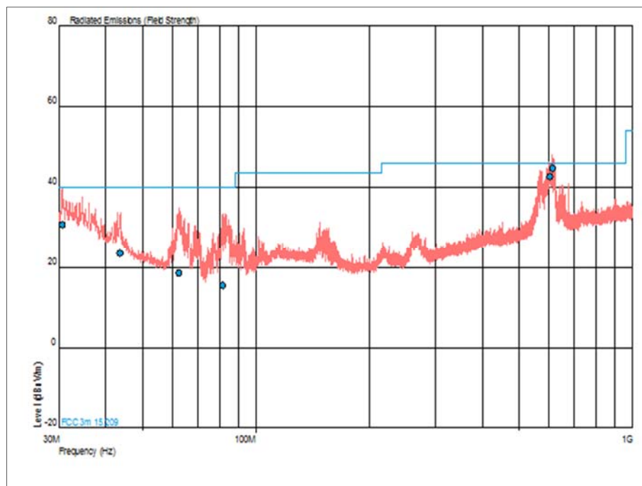
Figure 430 - U-NII 2c - 5500 MHz - 30 MHz to 1 GHz - Horizontal and Vertical
