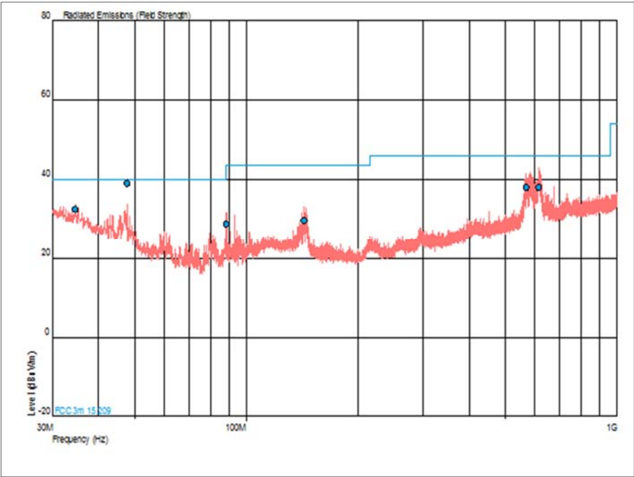
Figure 438 - U-NII 2c - 5700 MHz - 30 MHz to 1 GHz - Horizontal and Vertical
