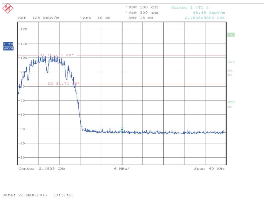
Figure 126 - Data Rate with Highest Power and Widest Bandwidth, 1 Mbps, 2462 MHz, Measured Frequency 2483.5 MHz
