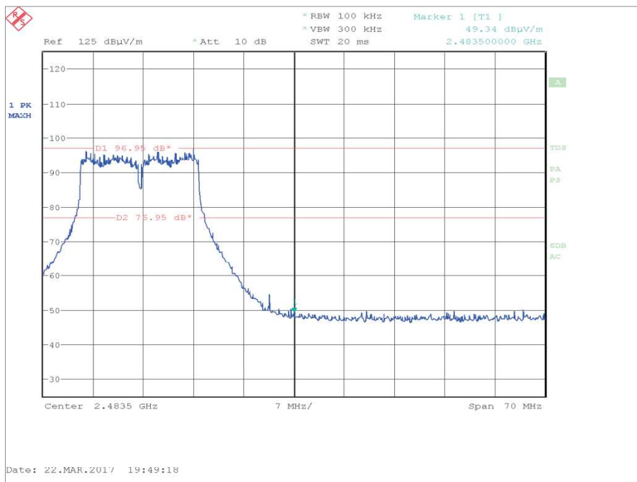
Figure 128 - Data Rate with Highest Power, 6 Mbps, 2462 MHz, Measured Frequency 2483.5 MHz
