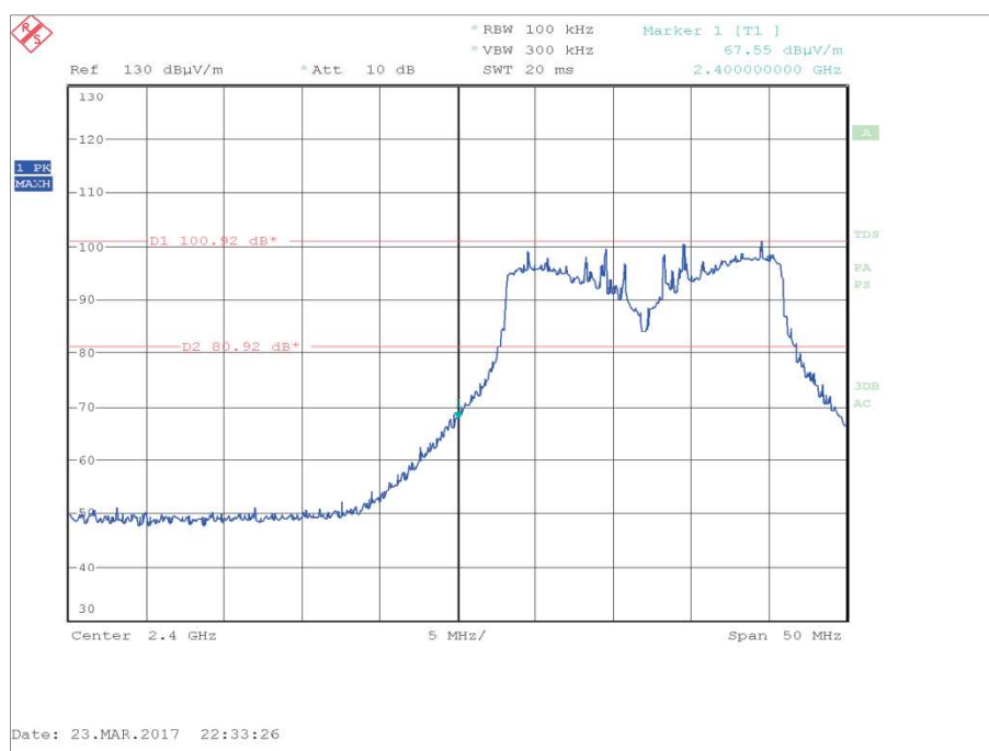
Figure 117 - MCS with Highest Power, MCS0, 2412 MHz, Measured Frequency 2400.0 MHz
