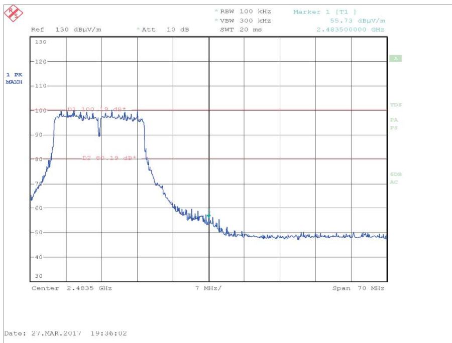
Figure 104 - MCS with Highest Power, MCS0, 2462 MHz, Measured Frequency 2483.5 MHz
