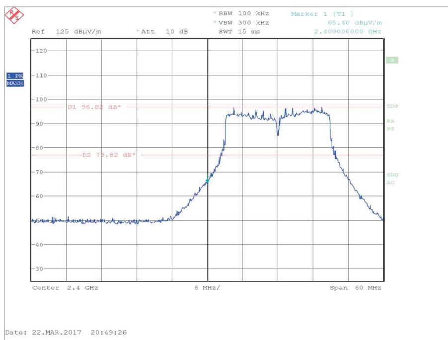
Figure 131 - MCS with Highest Power, MCS0, 2412 MHz, Measured Frequency 2400.0 MHz
