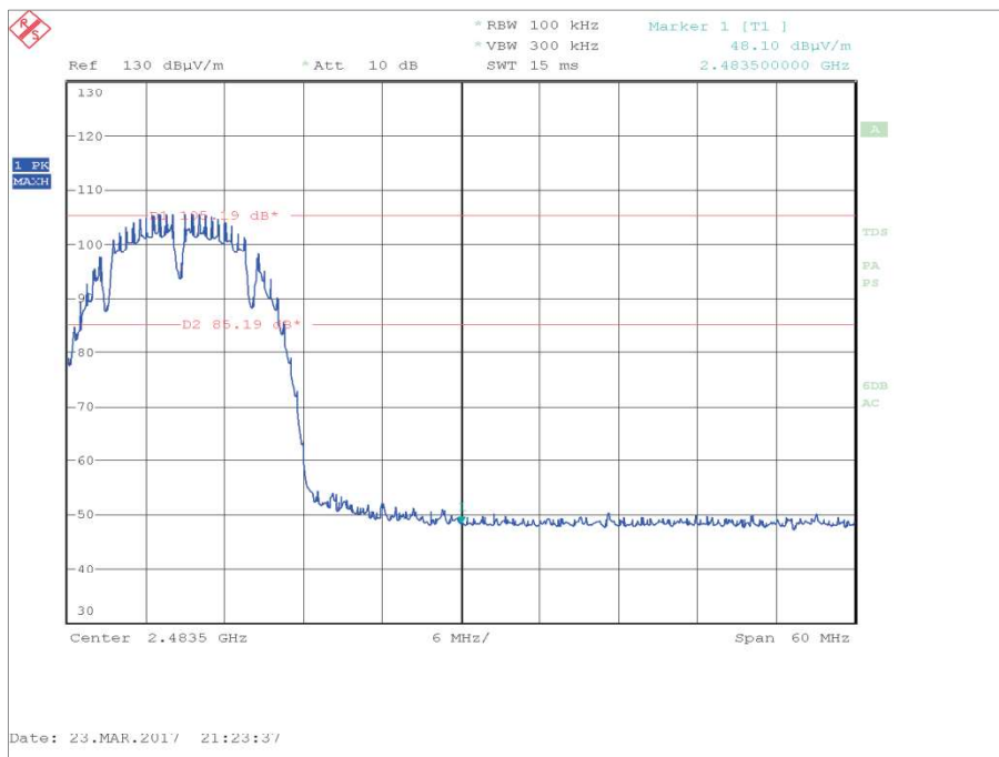
Figure 112 - Data Rate with Highest Power and Widest Bandwidth, 1 Mbps, 2462 MHz, Measured Frequency 2483.5 MHz
