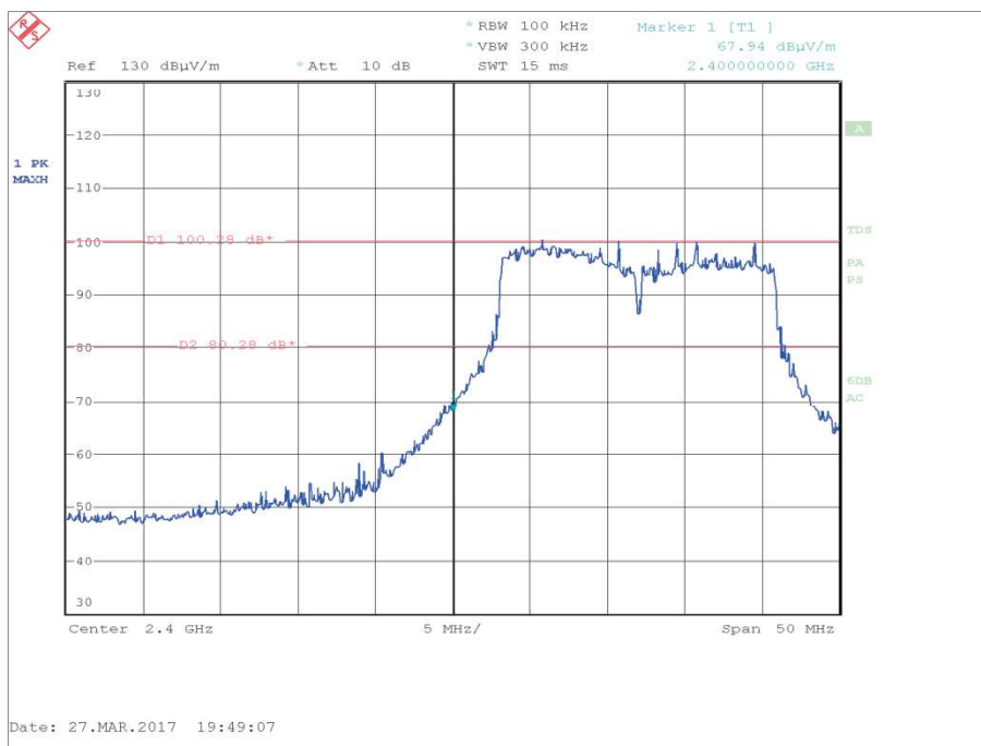
Figure 105 - MCS with Widest Bandwidth, MCS2, 2412 MHz, Measured Frequency 2400.0 MHz
