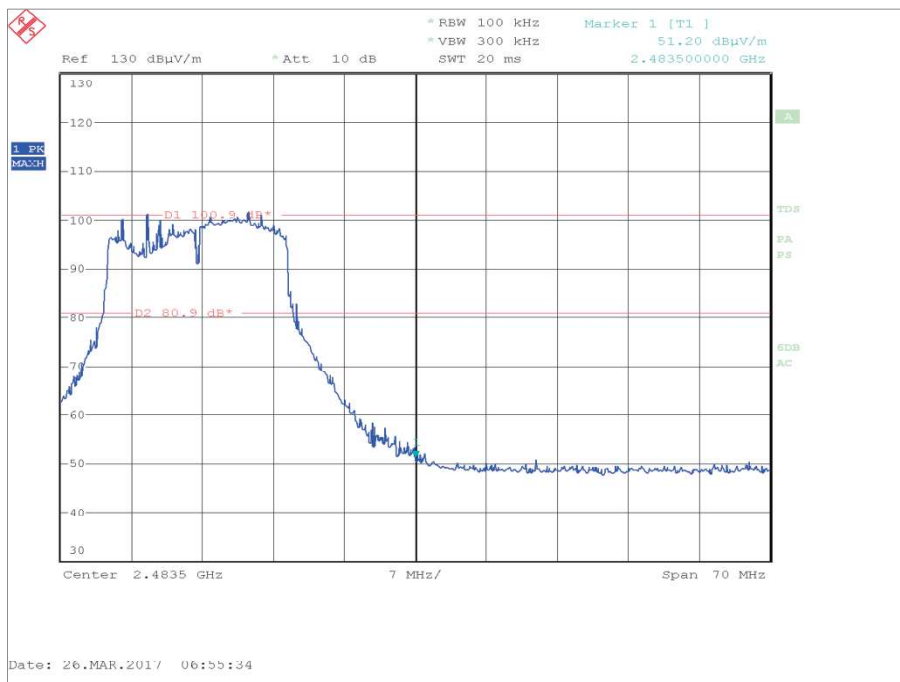
Figure 120 - MCS with Widest Bandwidth, MCS2, 2462 MHz, Measured Frequency 2483.5 MHz
