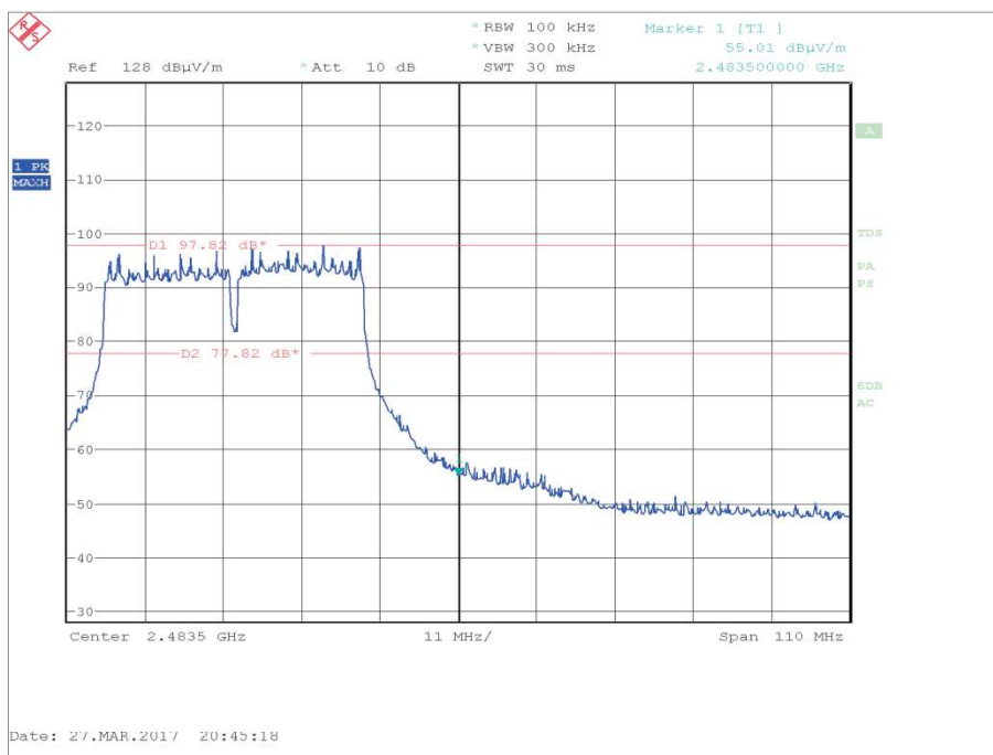
Figure 108 - MCS with Highest Power, MCS8, 2452 MHz, Measured Frequency 2483.5 MHz
