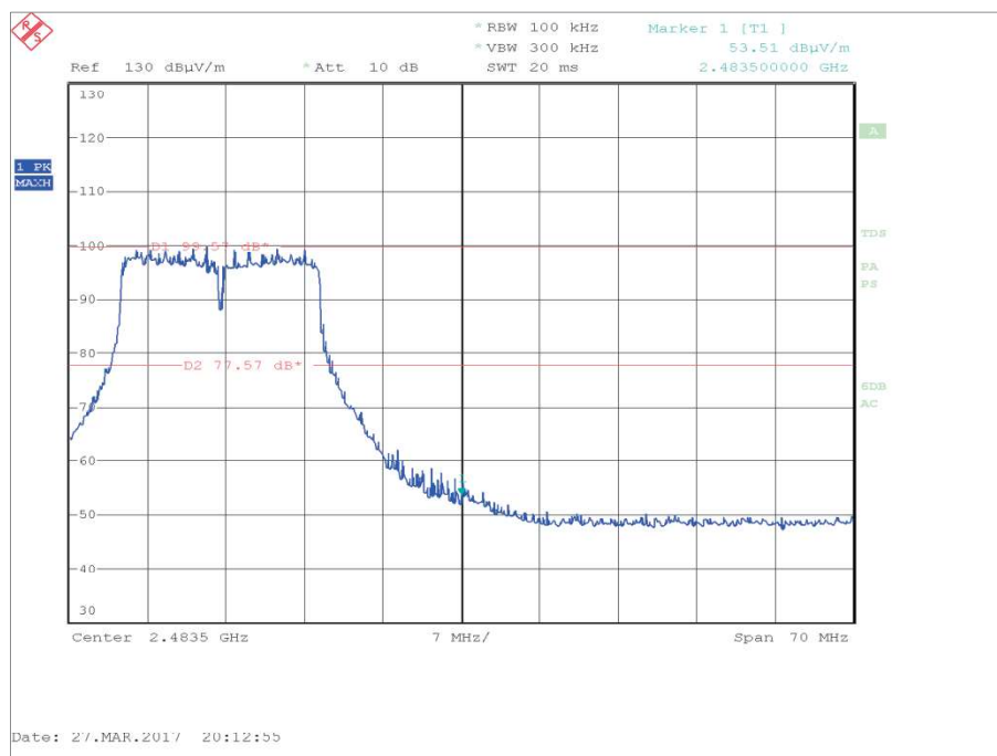
Figure 106 - MCS with Widest Bandwidth, MCS2, 2462 MHz, Measured Frequency 2483.5 MHz
