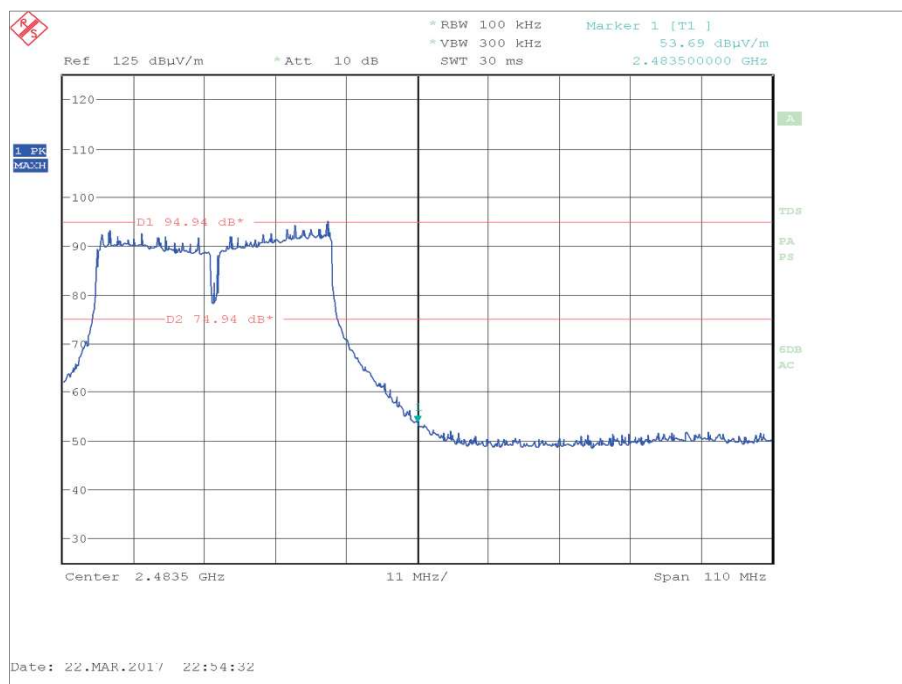
Figure 138 - MCS with Widest Bandwidth, MCS3, 2452 MHz, Measured Frequency 2483.5 MHz
