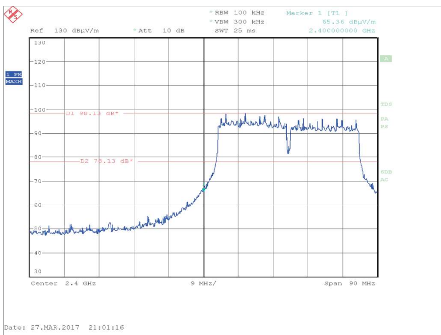
Figure 109 - MCS with Widest Bandwidth, MCS3, 2422 MHz, Measured Frequency 2400.0 MHz
