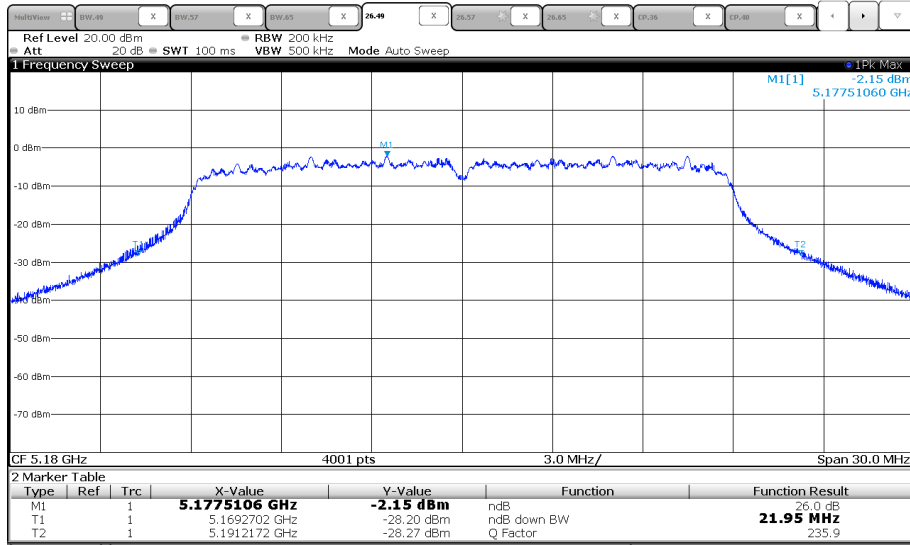
Channel 36 (5180 MHz)
