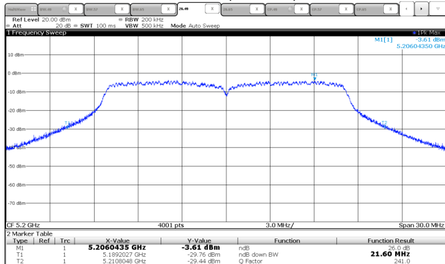
Channel 40 (5200 MHz)
