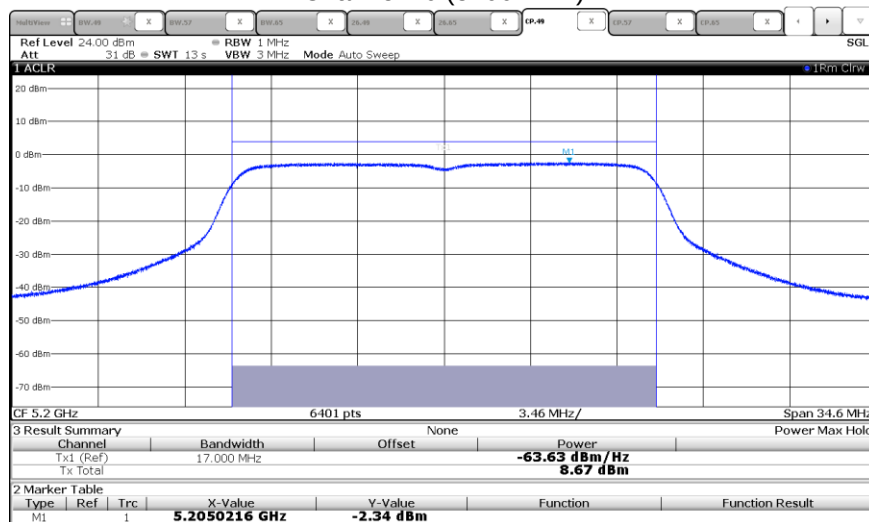
Channel 40 (5200 MHz)
