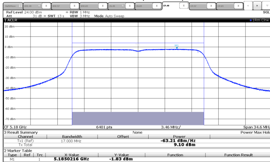
Channel 36 (5180 MHz)
