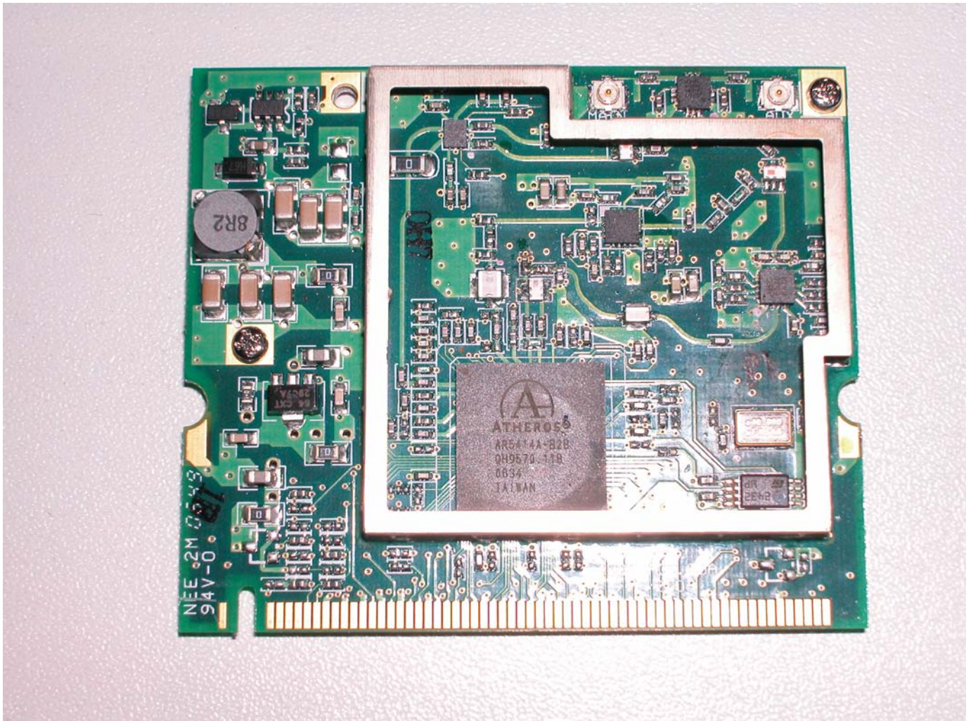
EAP Internal View Module without shielding
