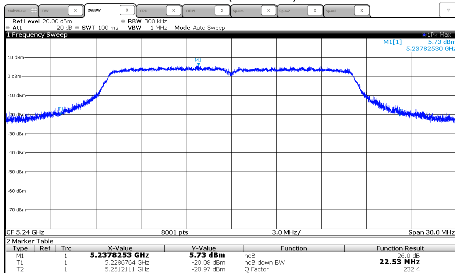
Channel 48 (5240 MHz)
