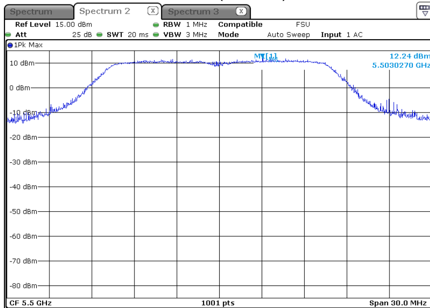
Channel 100 (5500 MHz)
