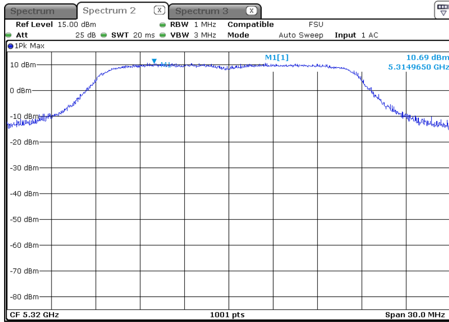
Channel 64 (5320 MHz)
