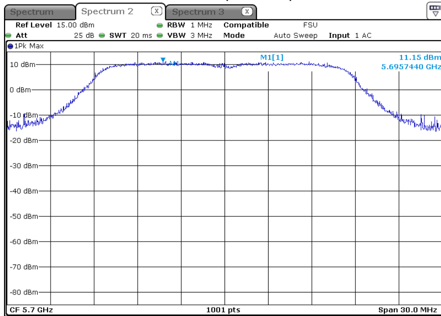
Channel 140 (5700 MHz)
