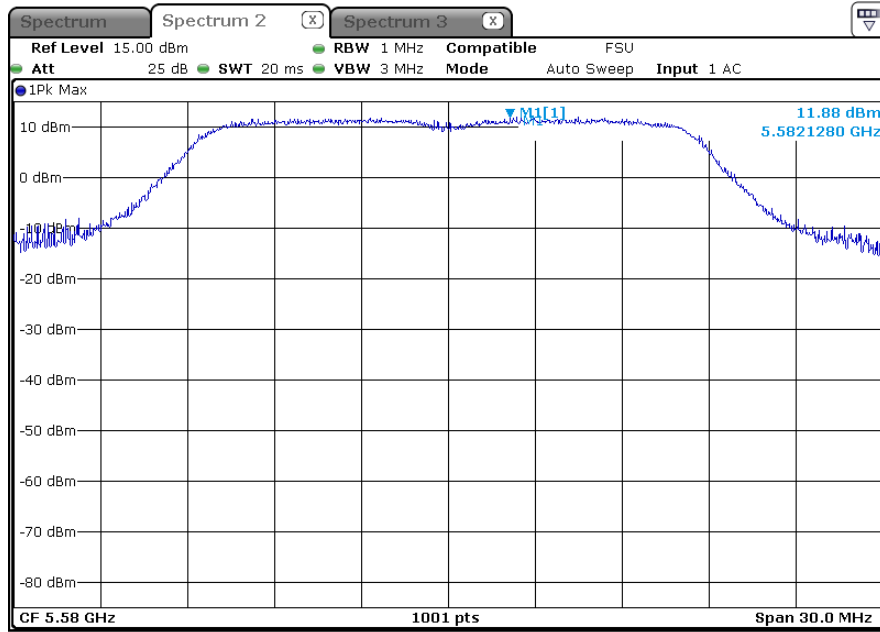
Channel 116 (5580 MHz)
