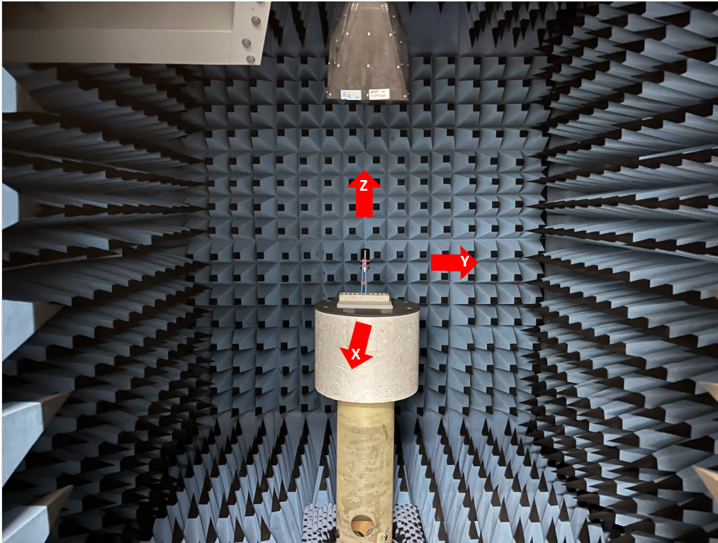
Photograph 3: EUT test setup 3D OTA test
