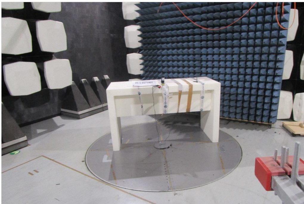
Photograph 5: EUT test setup in the semi anechoic chamber, overview_EUT elevation 0°
