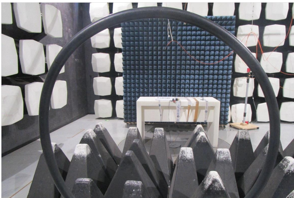
Photograph 7: EUT H-Field test setup in the semi anechoic chamber, overview
