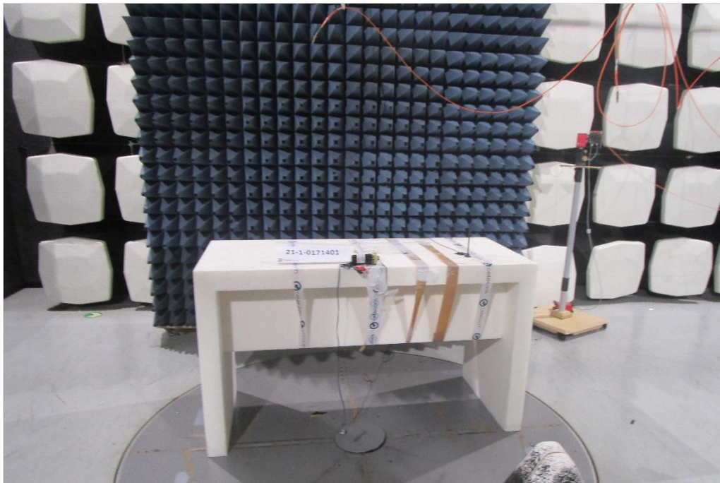
Photograph 6: EUT H-Field test setup in the semi anechoic chamber, close up view
