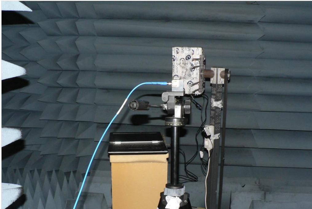
Photograph 3: EUT test setup in the fully anechoic chamber > 15 GHz, overview
