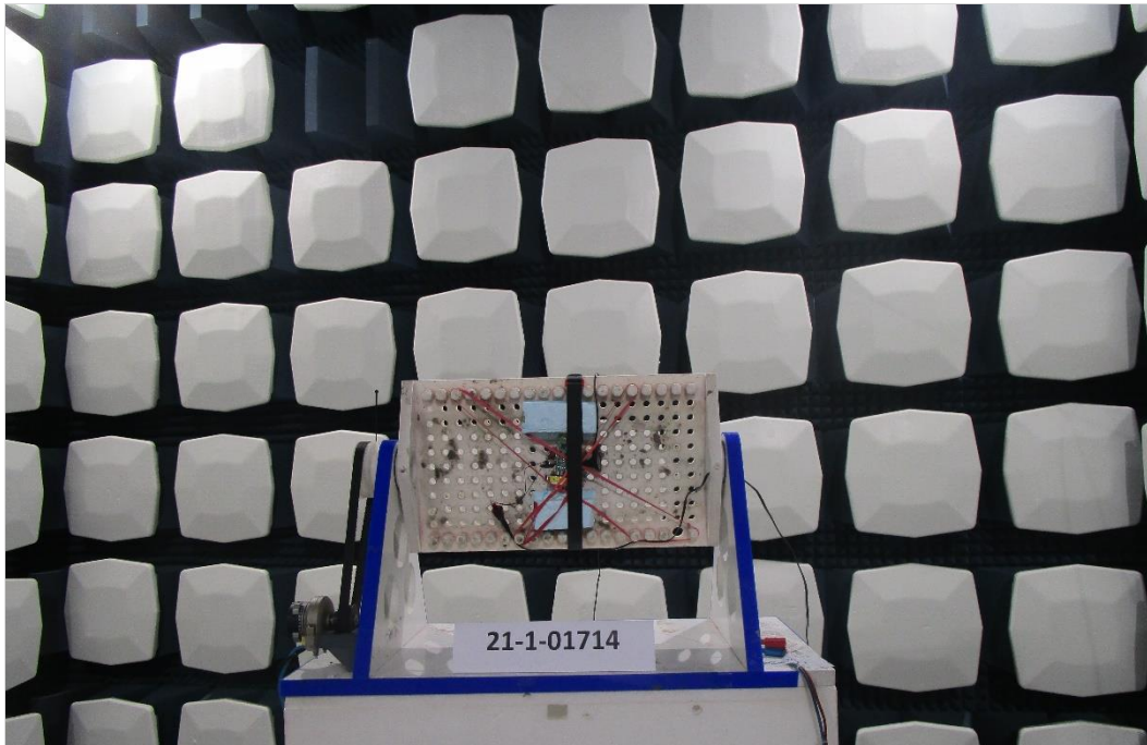
Photograph 1: EUT test setup in the fully anechoic chamber 1-15GHz, close up view
