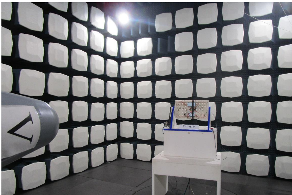
Photograph 2: EUT test setup in the fully anechoic chamber 1-15 GHz, overview
