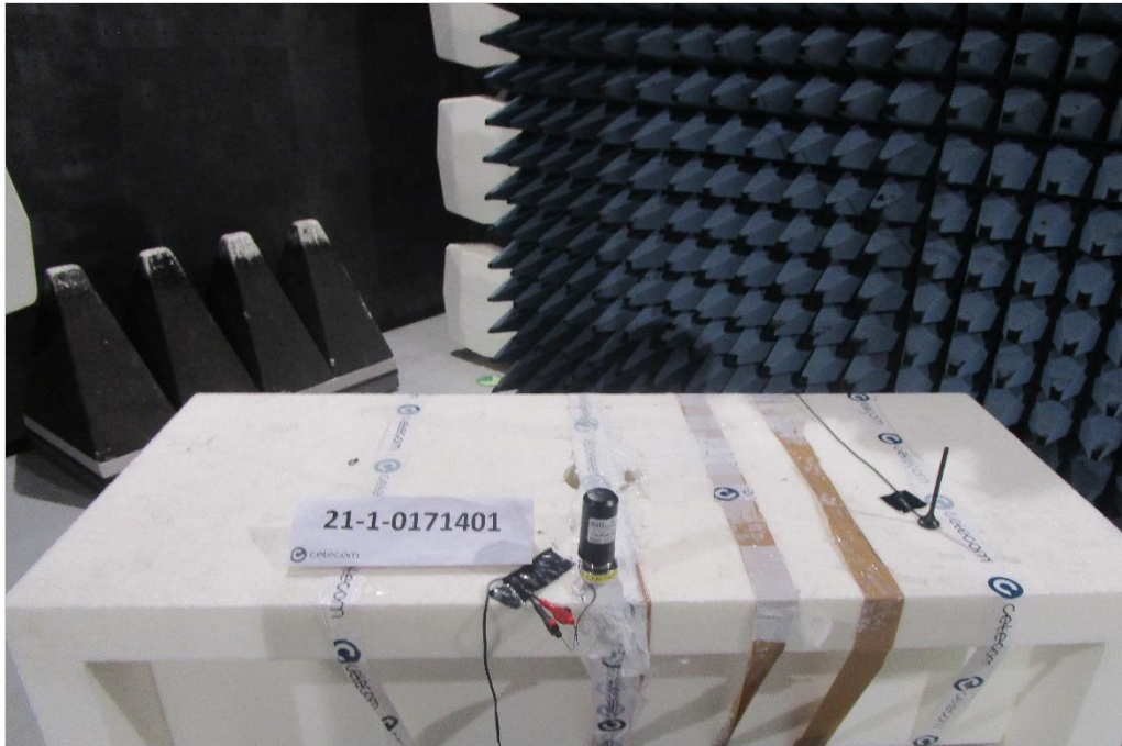
Photograph 4: EUT test setup in the semi anechoic chamber, close up view_EUT elevation 0°
