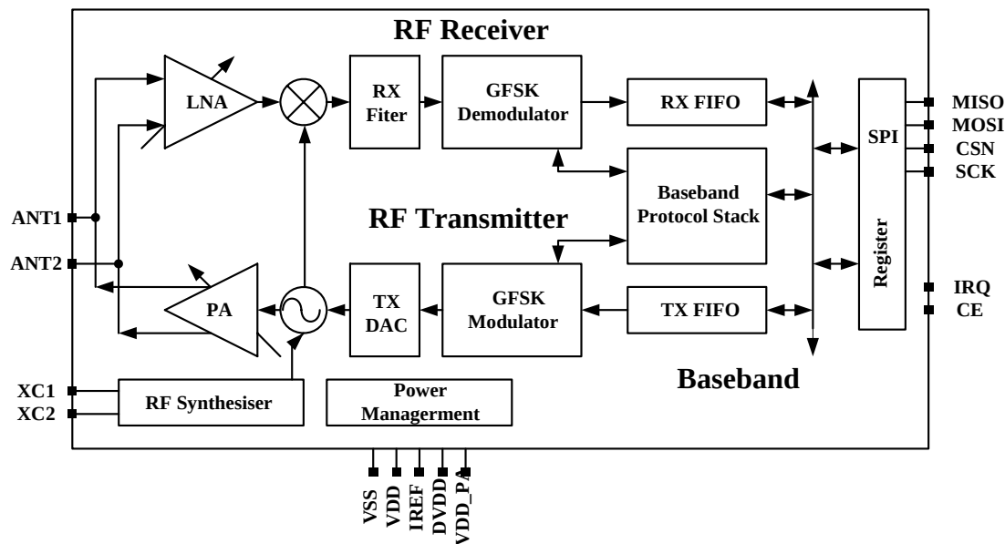
Figure 1 X2400 Block Diagram
