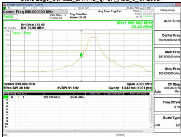
Band Edge Band12 1.4MHz QPSK RB1 0 CH23017
