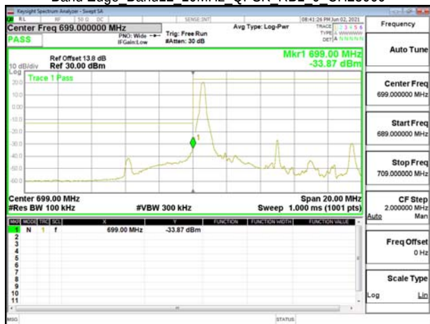
Band Edge Band12 10MHz QPSK RB1 0 CH23060
