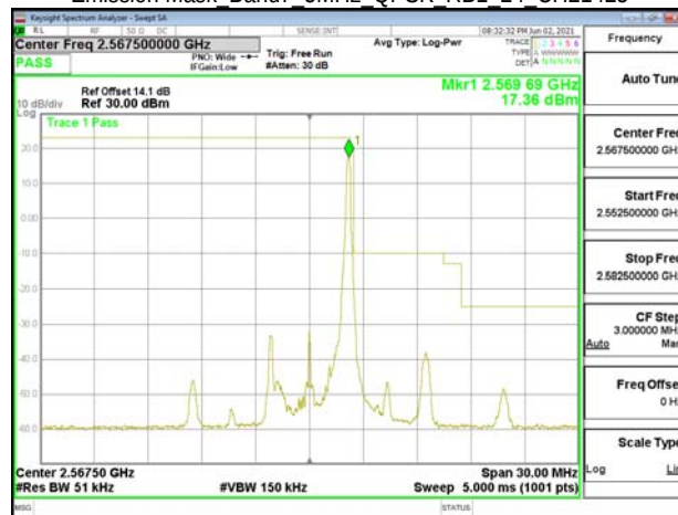
Emission Mask Band7 5MHz QPSK RB1 24 CH21425
