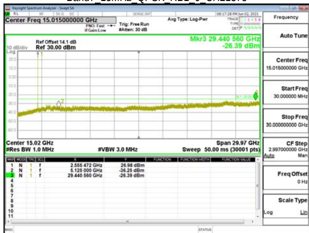
Band7 15MHz QPSK RB1 0 CH21375
