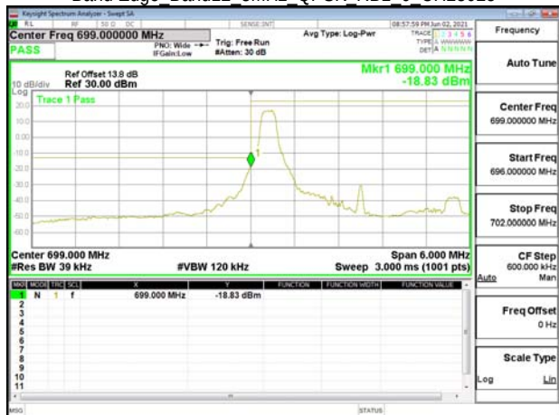
Band Edge Band12 3MHz QPSK RB1 14 CH23165
