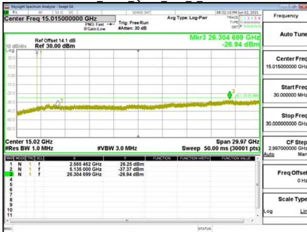
Band7 5MHz QPSK RB1 0 CH21425
