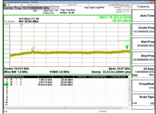
Band2 3MHz QPSK RB1 0 CH19185
