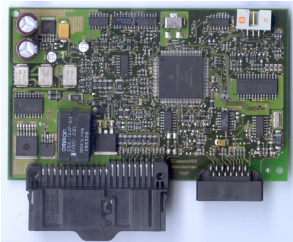
CAS E8X/9X (top view of PCB)
