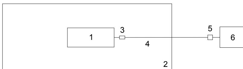
Figure 3: Measurement setup for testing on antenna connector
