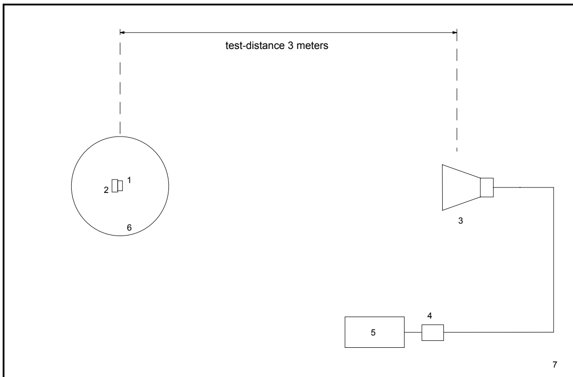
Figure 2: Measurement setup for radiated emission test above 1 GHz
