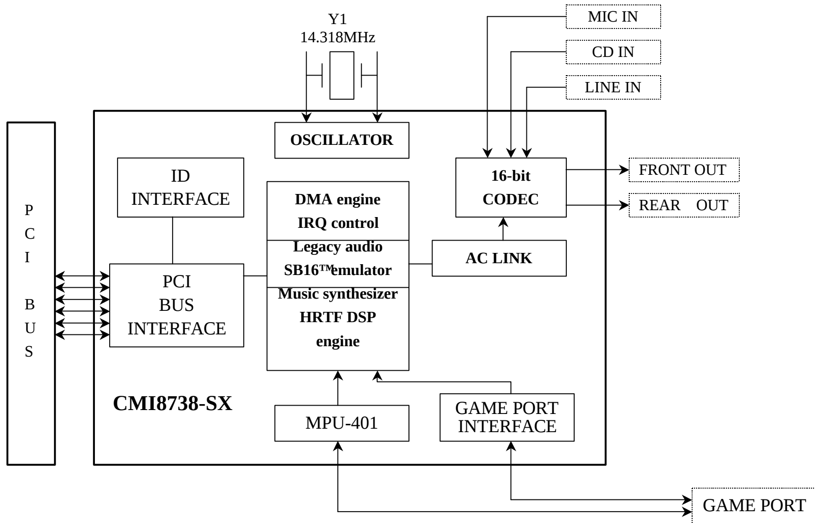
A521-W00 BLOCK DIAGRAM
