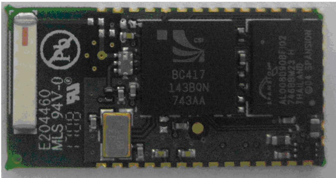
Component Side
