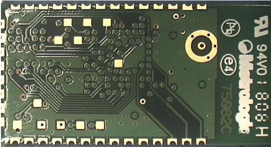
Back Side
