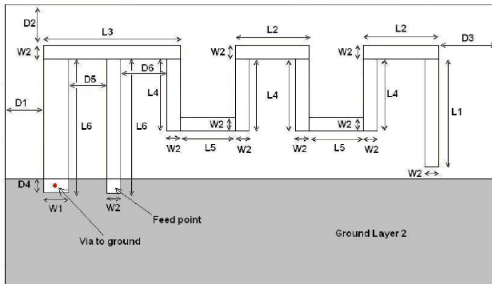
Figure 3: Antenna Dimensions
