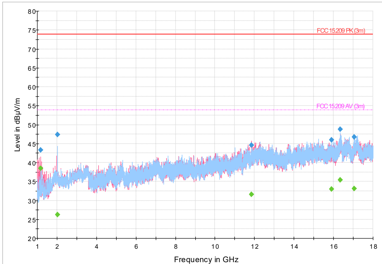
Figure 8.2-9: Radiated spurious emissions, 802.11n-HT20, MCS0, 1-18 GHz spectral plot (2437 MHz)
