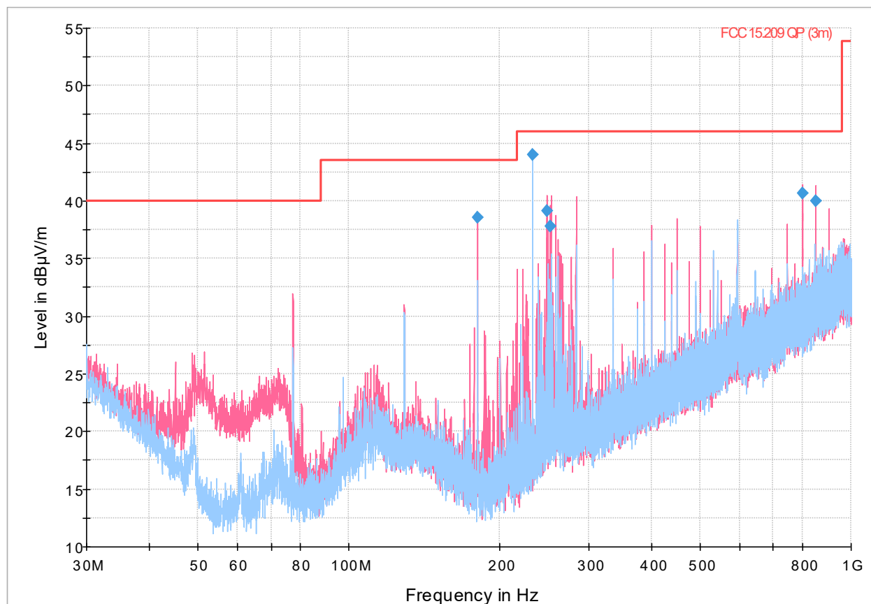
Figure 8.2-8: Radiated spurious emissions, 802.11n-HT20, MCS0, 30-1000 MHz spectral plot (2437 MHz)
