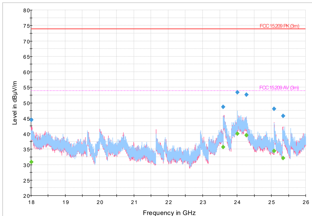
Figure 8.2-10: Radiated spurious emissions, 802.11n-HT20, MCS0, 18-26 GHz spectral plot (2437 MHz)
