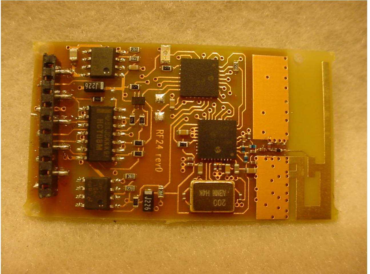
Figure 2: RF24 Front View – No Shield
