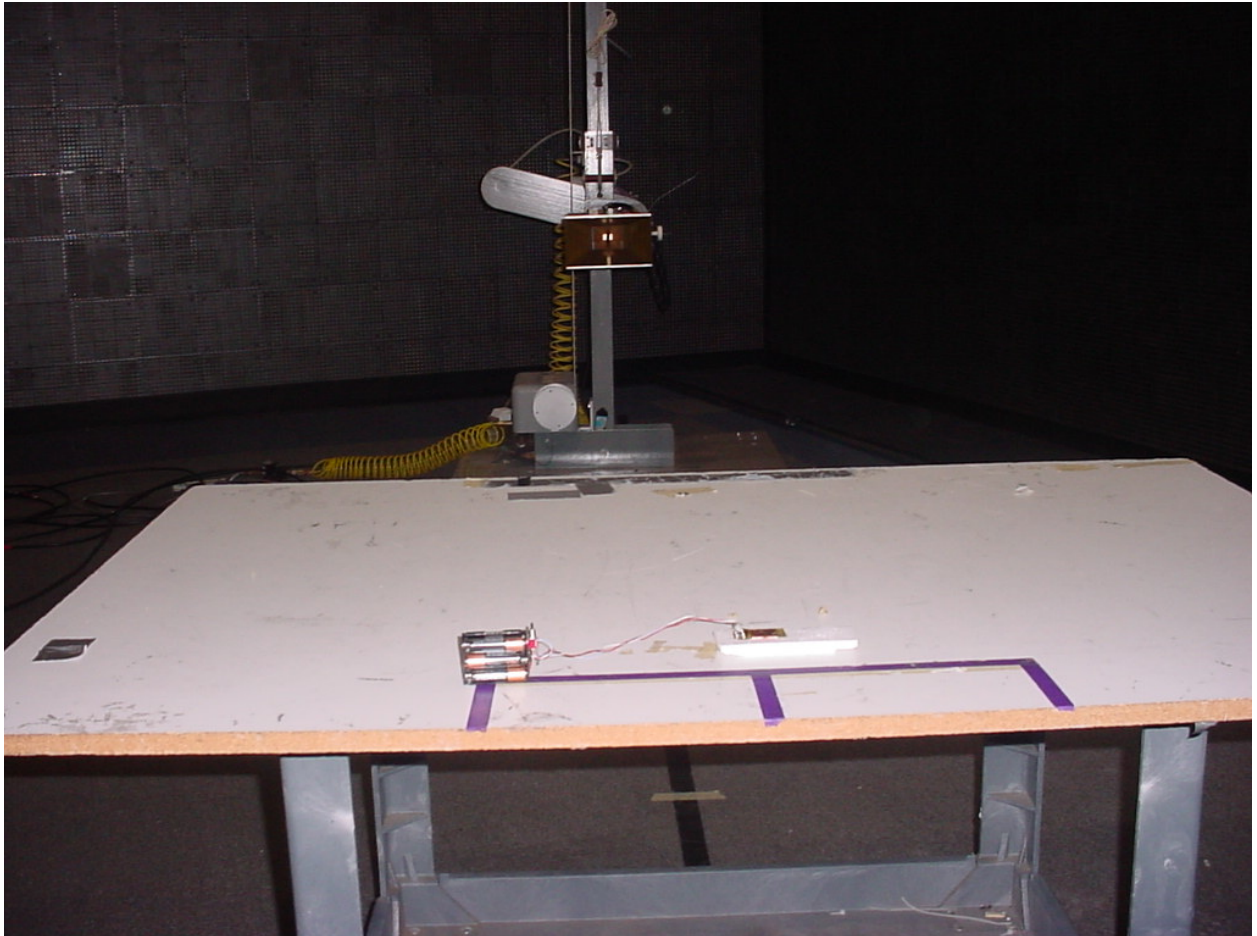
Figure 4: Test Setup Radiated Emissions – Intentional
