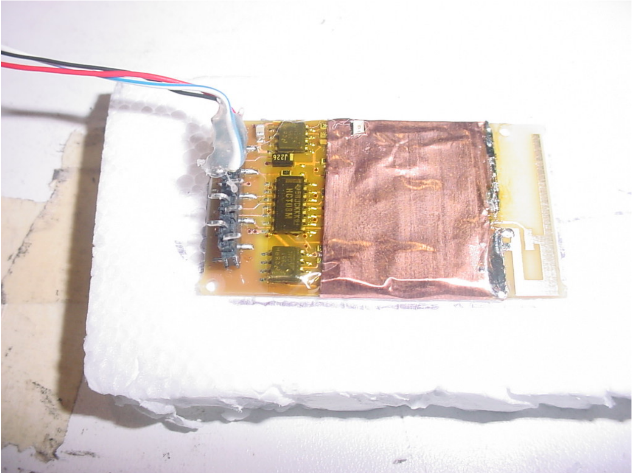
Figure 5: Test Setup Radiated Emissions - Intentional
