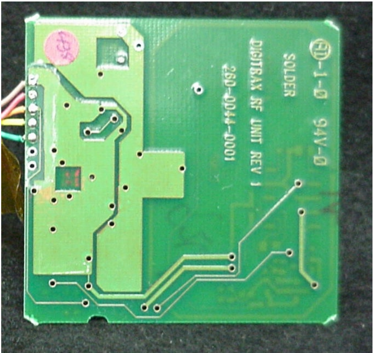
Photo 2. EUT, Bottom View of Transmitter Board
