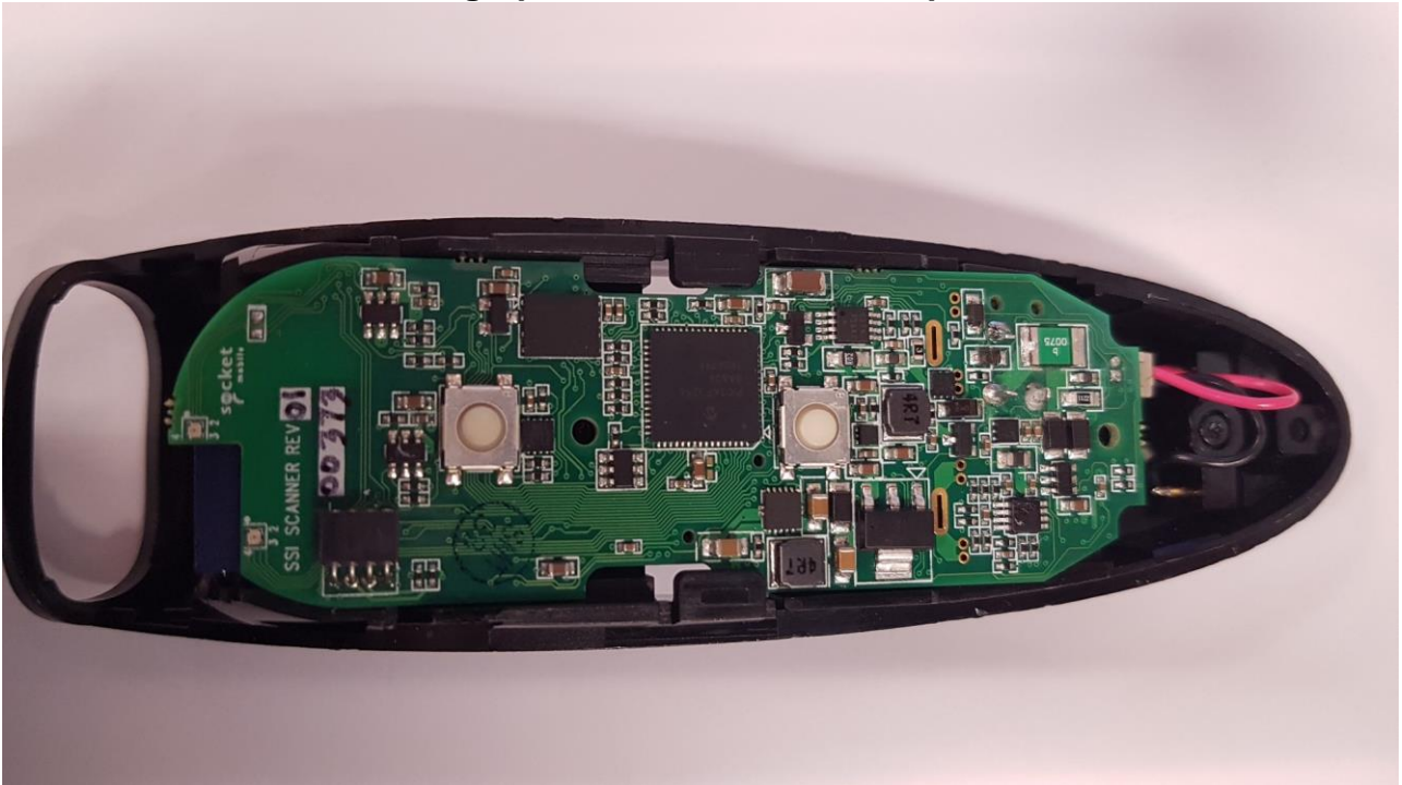
S700 Circuit Board – Rear View
