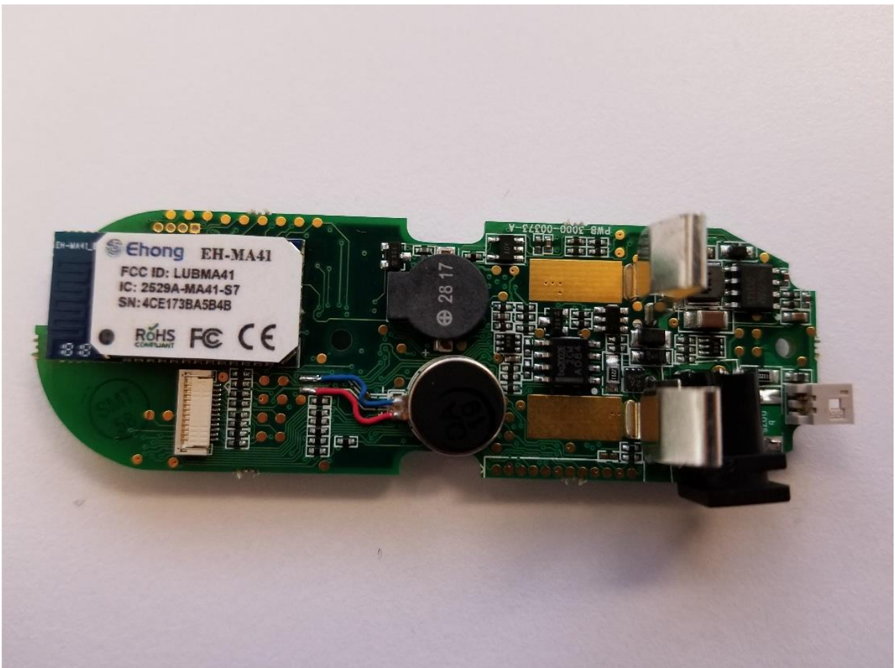
S700 Circuit Board – Rear View
