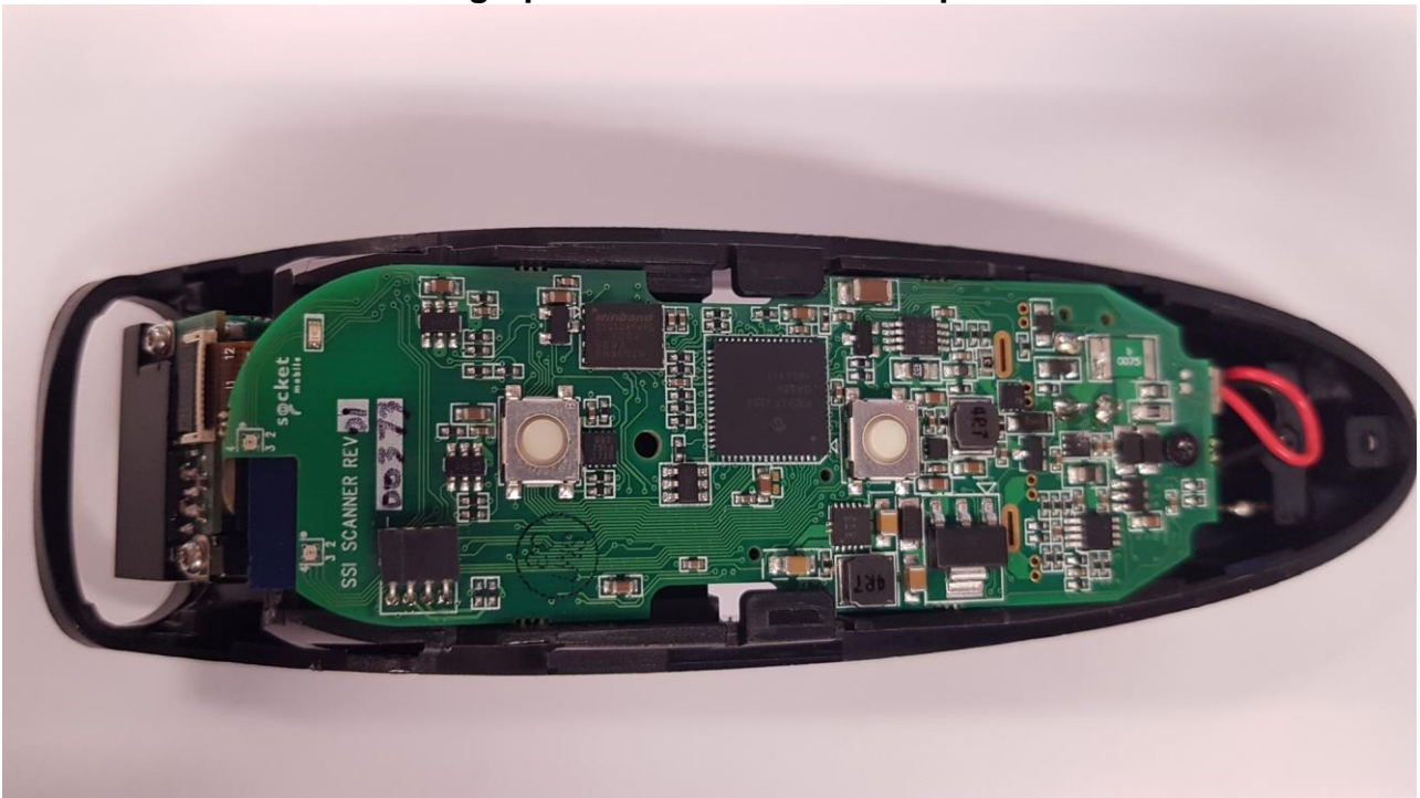
S730 Circuit Board – Rear View
