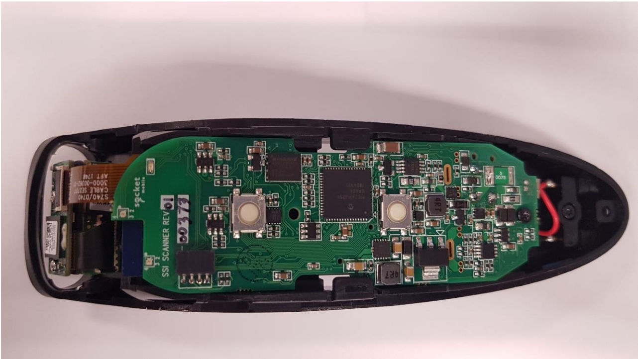
S740 Circuit Board – Rear View
