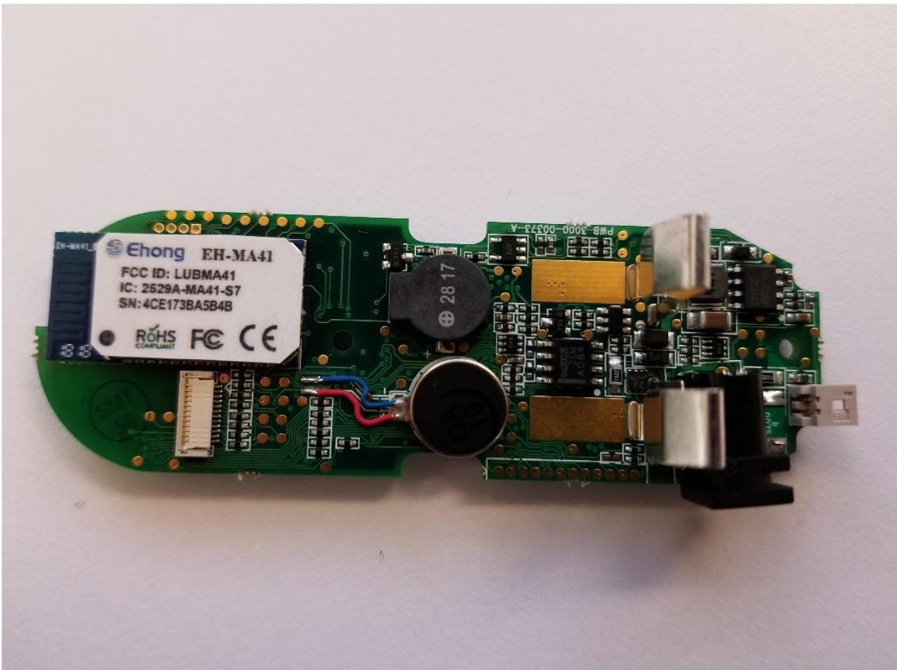
S740 Circuit Board – Rear View
