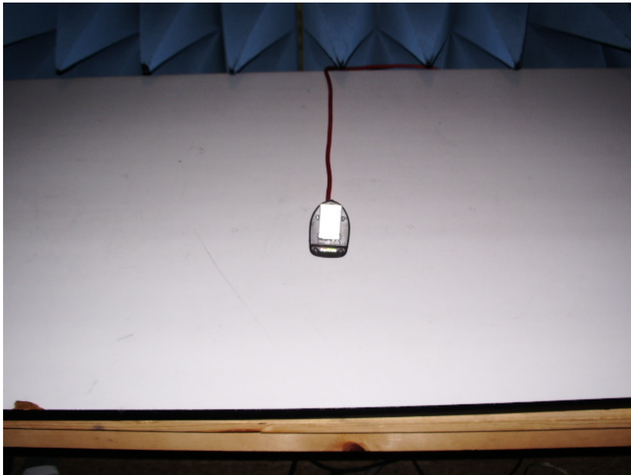
Line Conducted Emissions Setup (Battery Charger)
