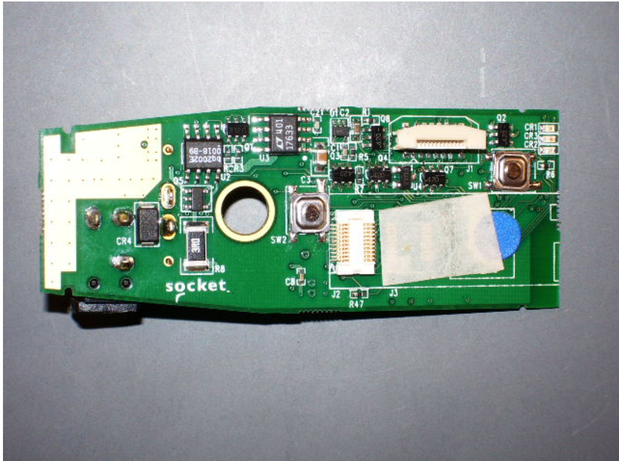
Main PCB – Top View
