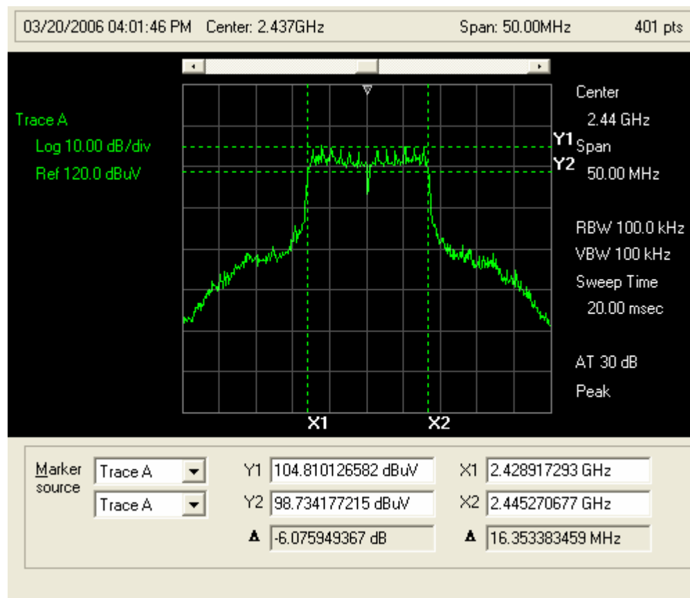
Plot 14: 6 dB BW 2437 MHz / 6 Mbit Modulation
