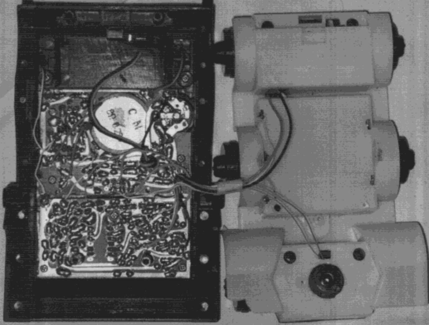
FCC ID: LU9-MGA921A Bottom View of the Printed Wiring Board
