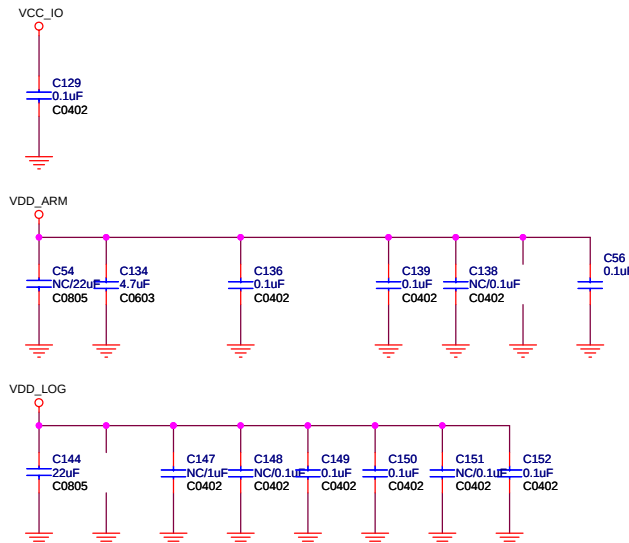
RK3188 CORE POWER FILTER
