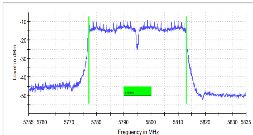
6 dB Bandwidth
