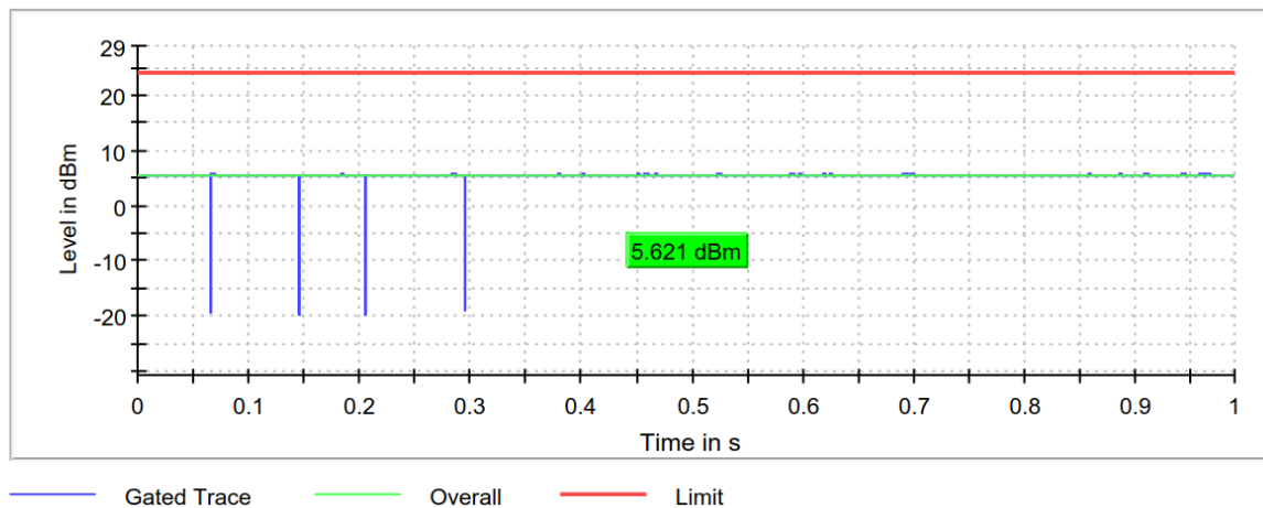
Gated Trace
