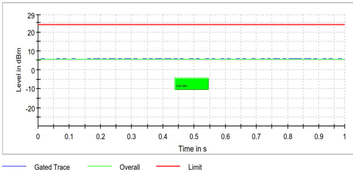
Gated Trace
