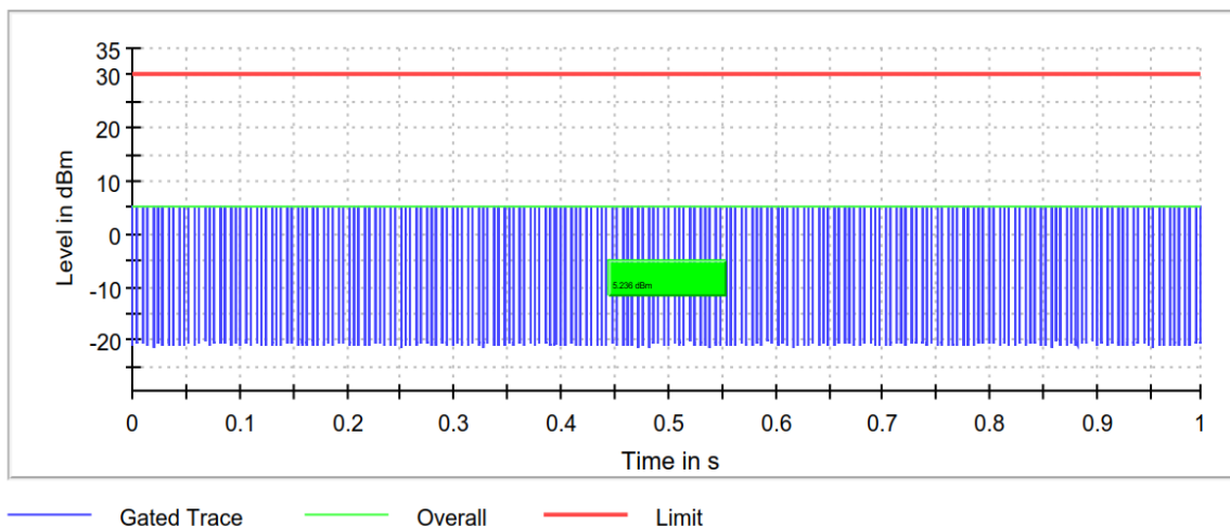
Gated Trace
