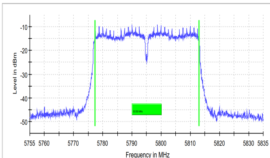
6 dB Bandwidth
