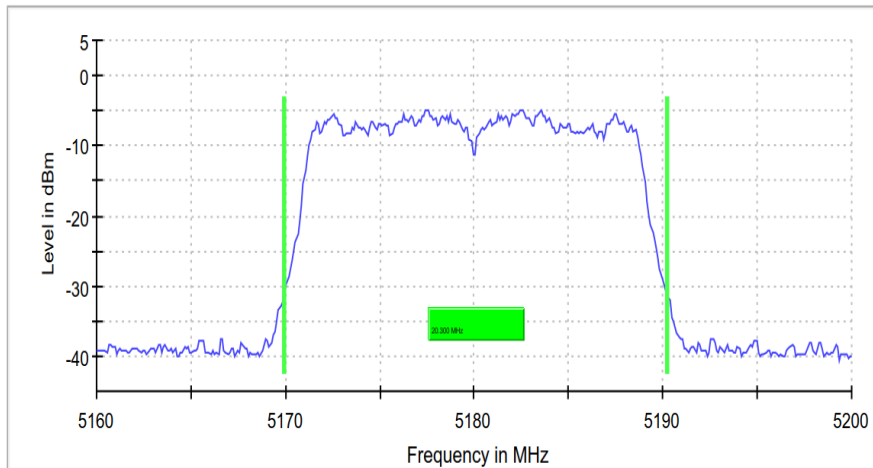
26 dB Bandwidth
