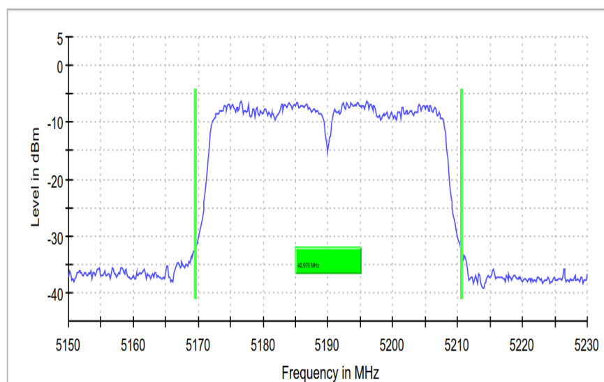
26 dB Bandwidth
