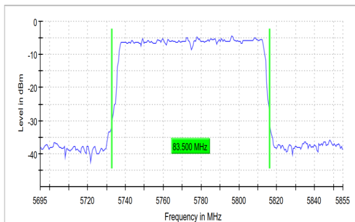
26 dB Bandwidth
