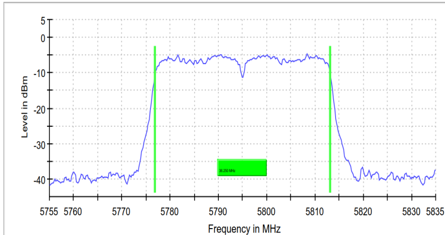
99 % Bandwidth
