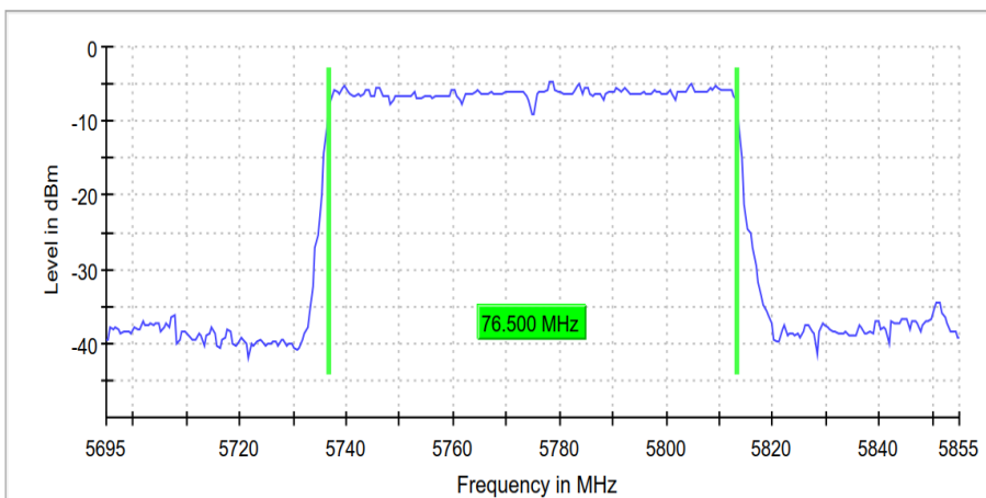
99 % Bandwidth
