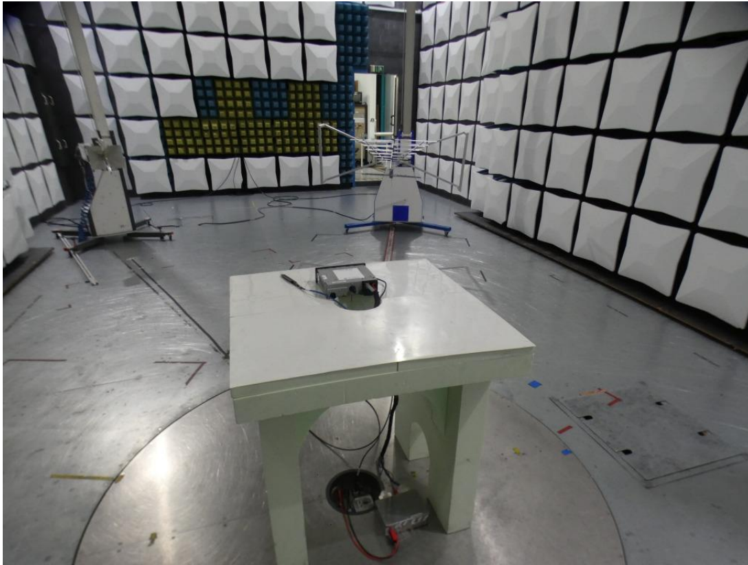
Photo 2: Test setup for radiated measurements (30 MHz – 1 GHz)
