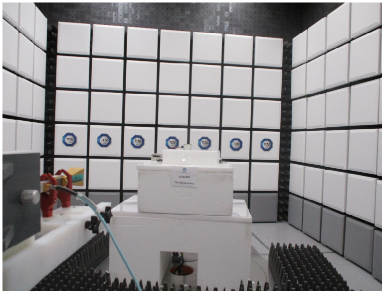
Radiated Emissions 75-110 GHz Rear
