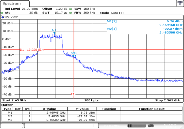
Channel 12 (2467MHz)
