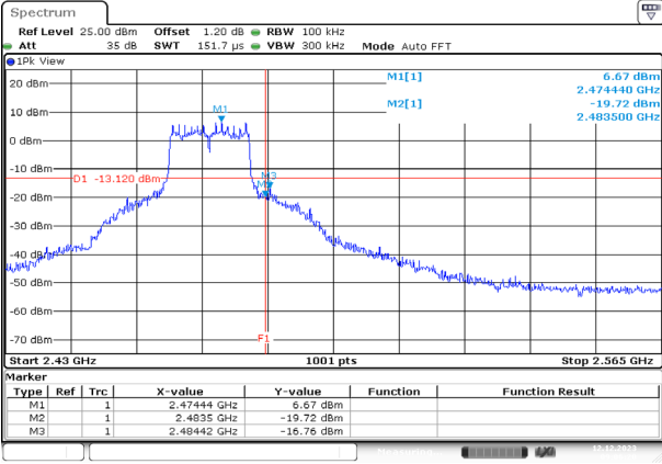
Channel 13 (2472MHz)
