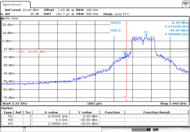
Channel 01 (2412MHz)
