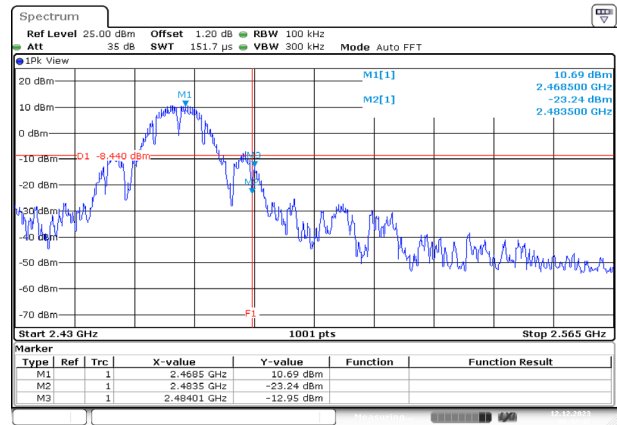
Channel 12 (2467MHz)
