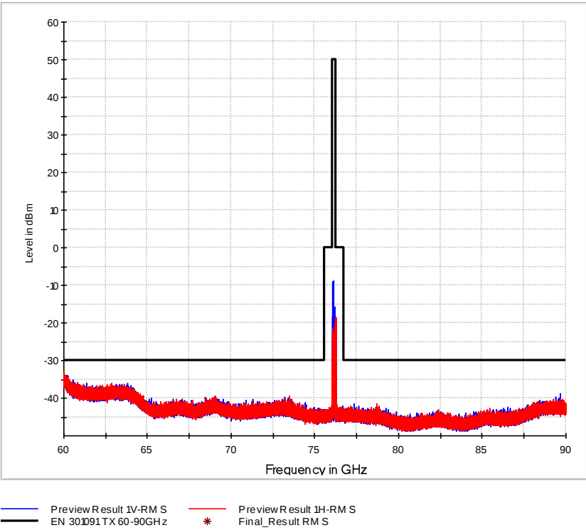
Plot shows intentional radar emission in 76-81 GHz Band
