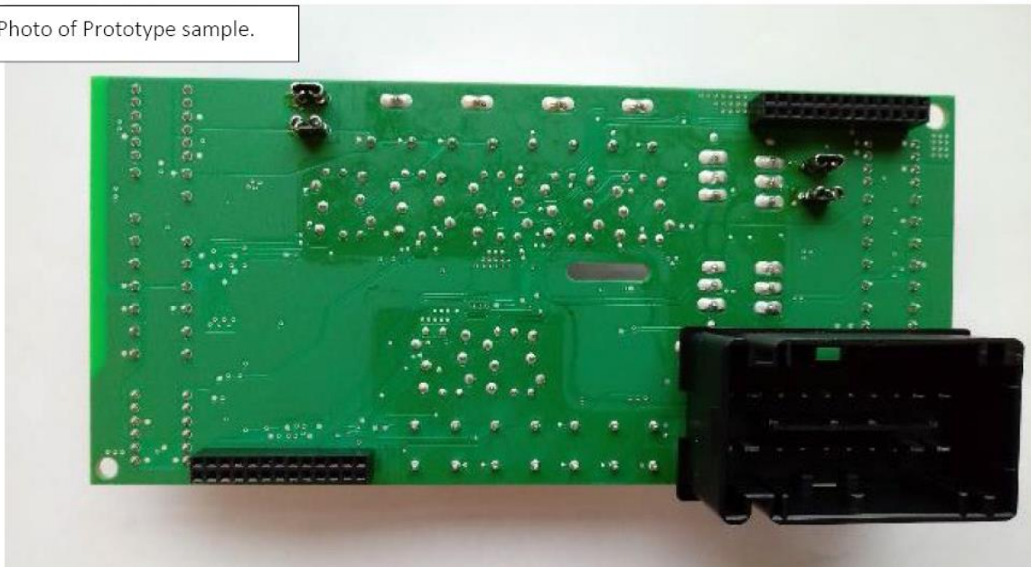
Figure 43: IBCM - power board bottom view
