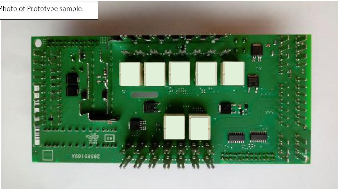
Figure 42: IBCM - power board top view
