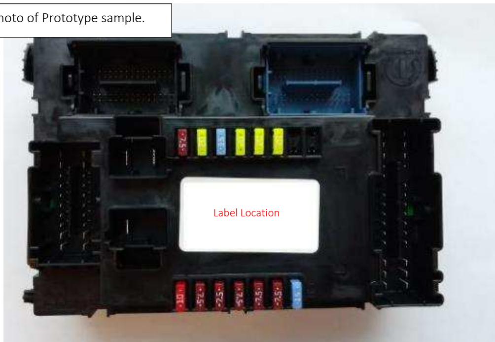
Figure 28: IBCM top view
