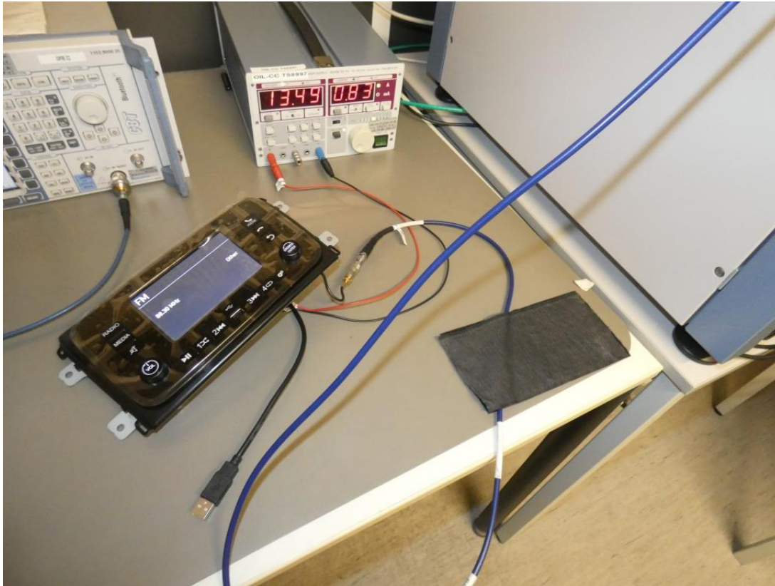
Photo 5: Test setup for conducted measurements on R&S TS8997
