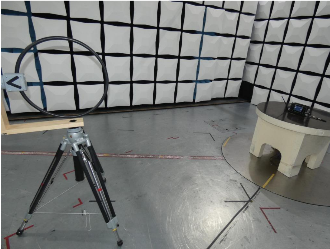
Photo 1: Test setup for radiated measurements ( 9 kHz - 30 MHz; FCC 15c247)
