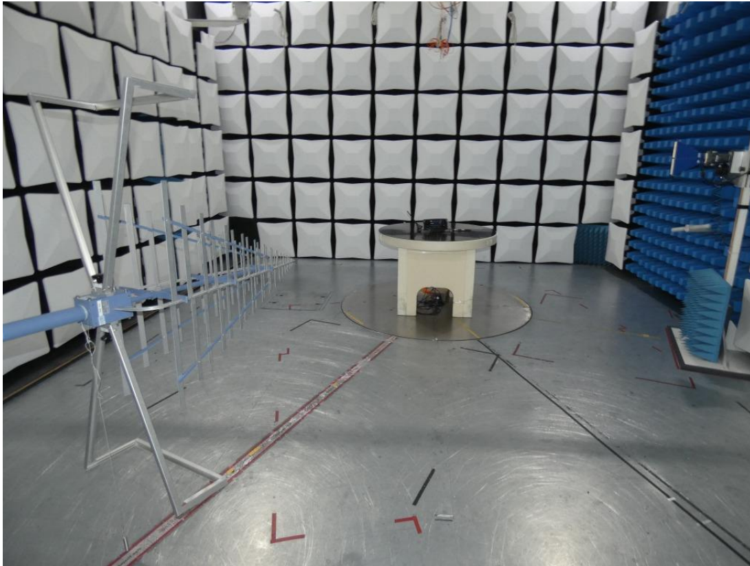
Photo 2: Test setup for radiated measurements (30 MHz - 1 GHz; FCC 15c247)
