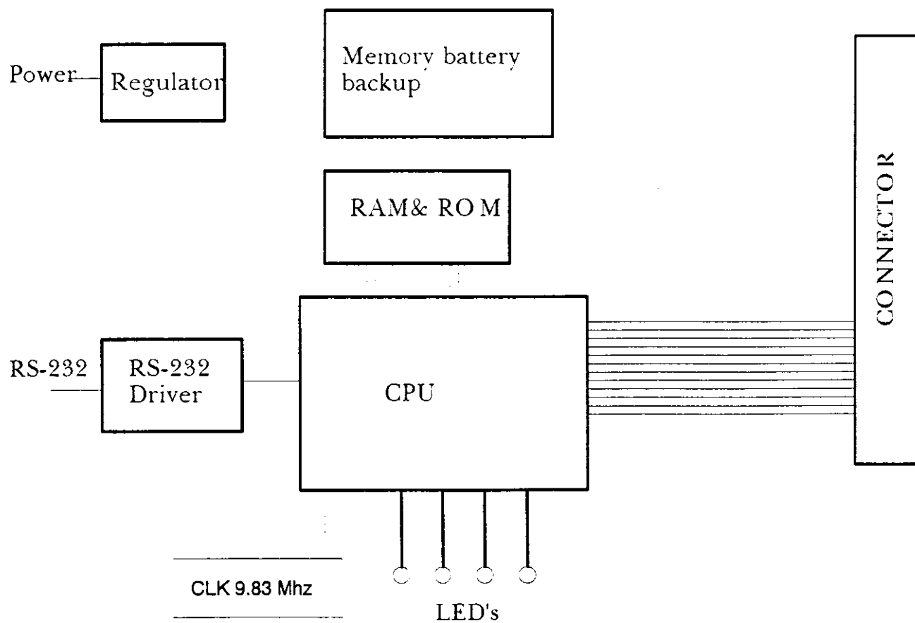
LAWNIIIP's Block Diagram
