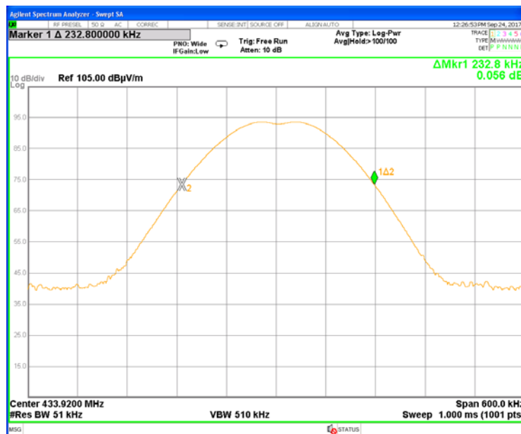
Plot # 9. Occupied bandwidth test result
