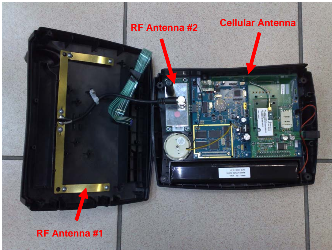
Figure 1: DCU-2010C-2 (Open)
