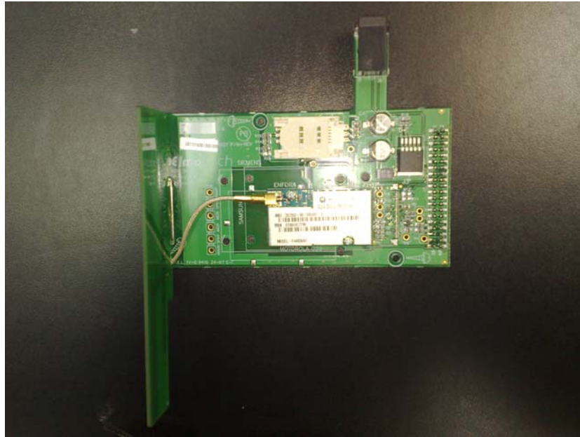
Figure 7: Cellular Module (Top)
