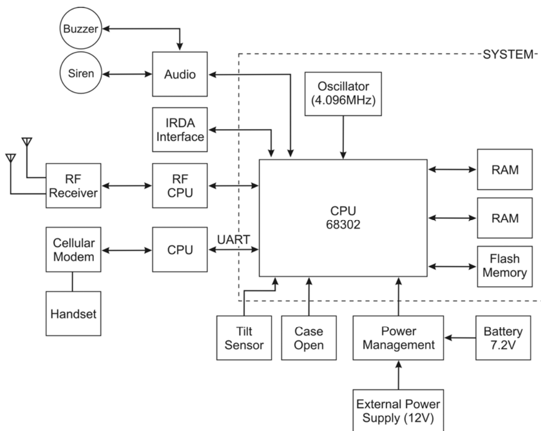
Figure 1. EUT block diagram
