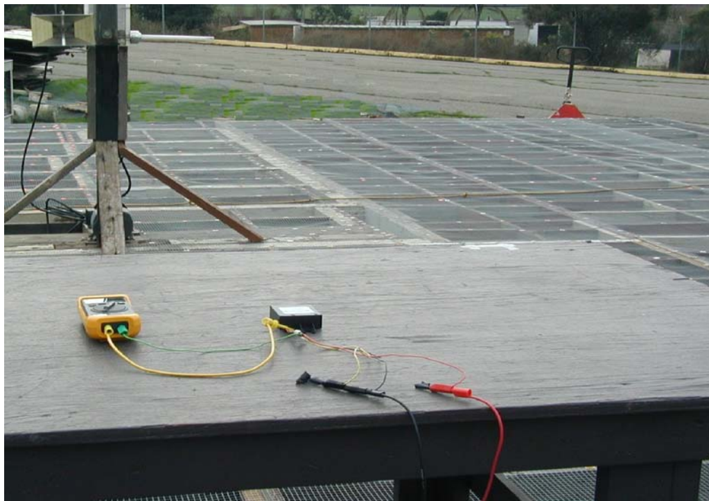
Figure 4: Test Set Up Photos – Spurious, Harmonics, and Restricted Test Set up (above 1GHz)
