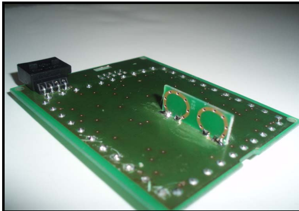
Figure 6: EUT Internal View 3
