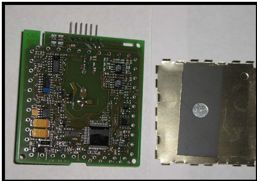
Figure 2: EUT Component View with shield off
