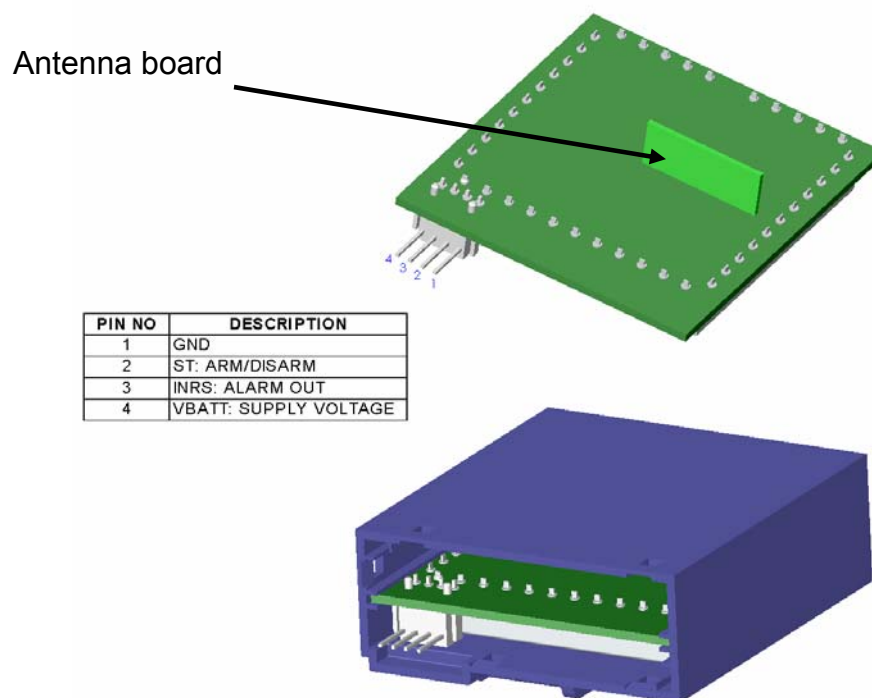
Figure 1 EUT Pin assignments
