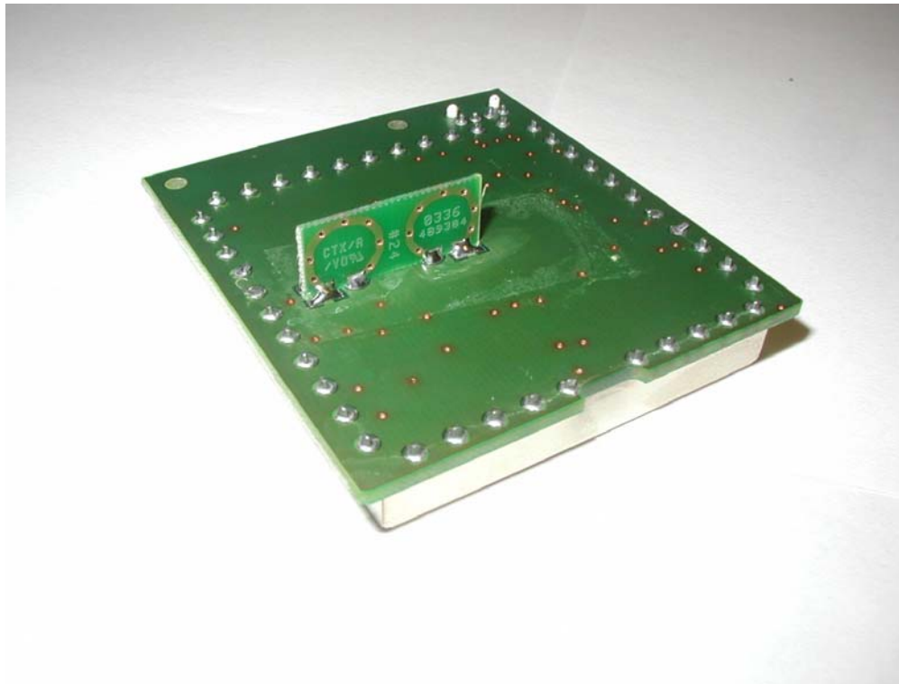
Figure 4 Antenna Board-Side 1
