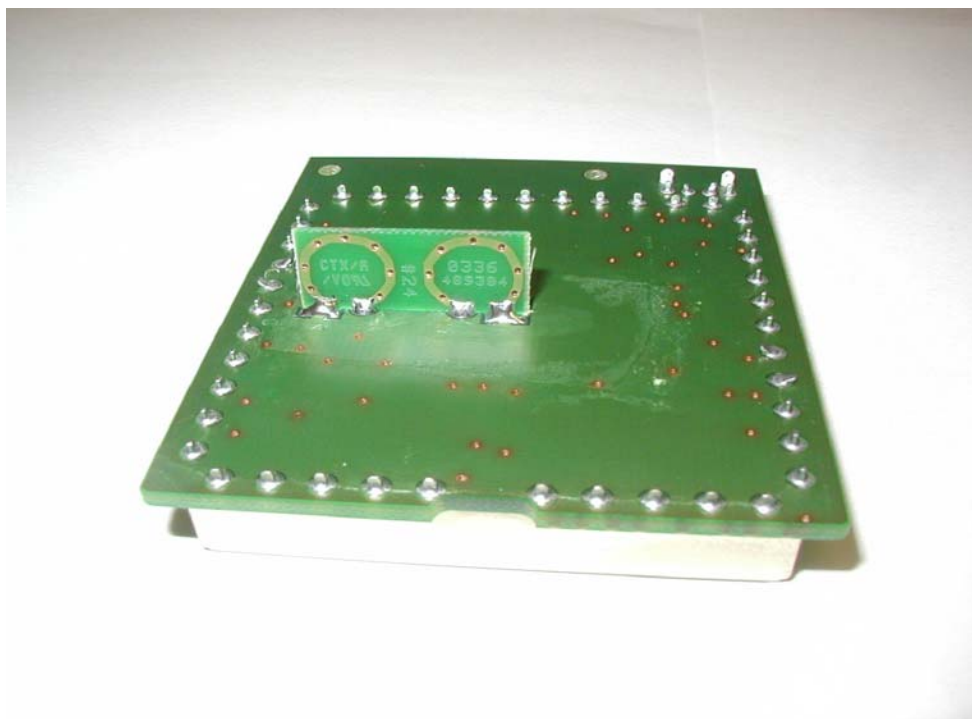
Figure 4: Antenna Board-Side
