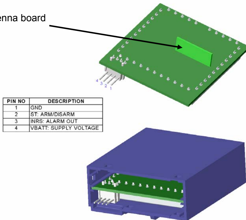
Figure 1 EUT Pin assignments
