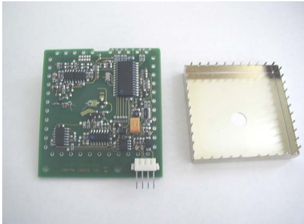
Figure 3: Component Side of board – no Cover Shield
