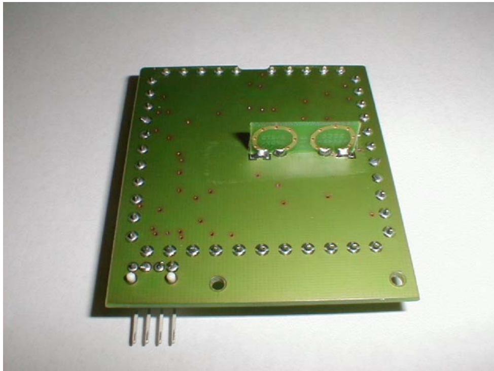
Figure 5: Antenna Board-Side 2
