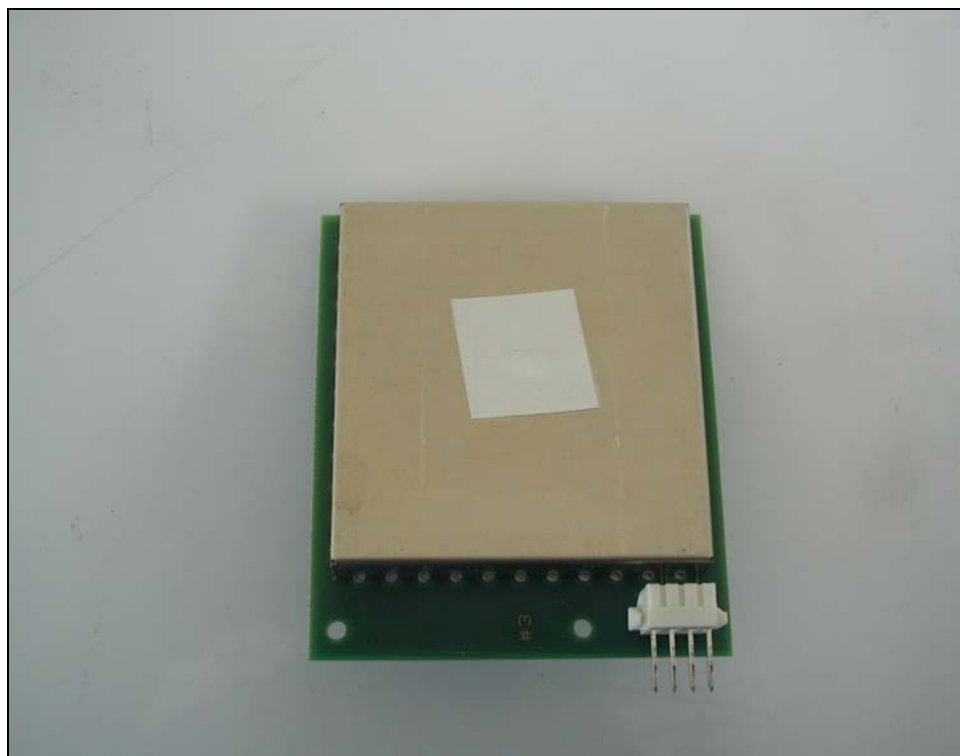
Figure 2: Component Side of Board with metal enclosure shield
