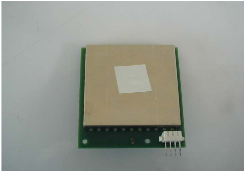
EUT Mainboard – Component Side View (with Shield Cover)
