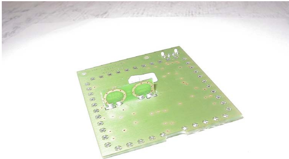
Antenna Board –Side1
