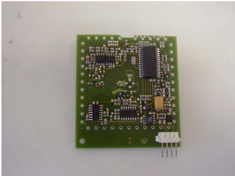
Mainboard – Component Side View (Shield Cover Removed)
