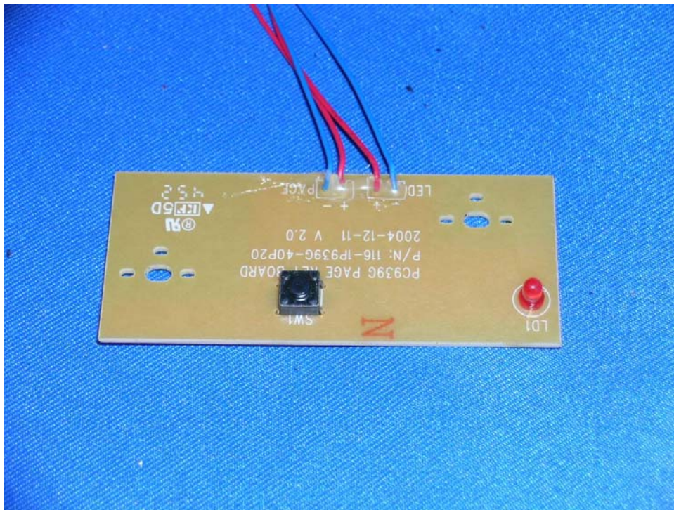
Base Page Key and LED front side
